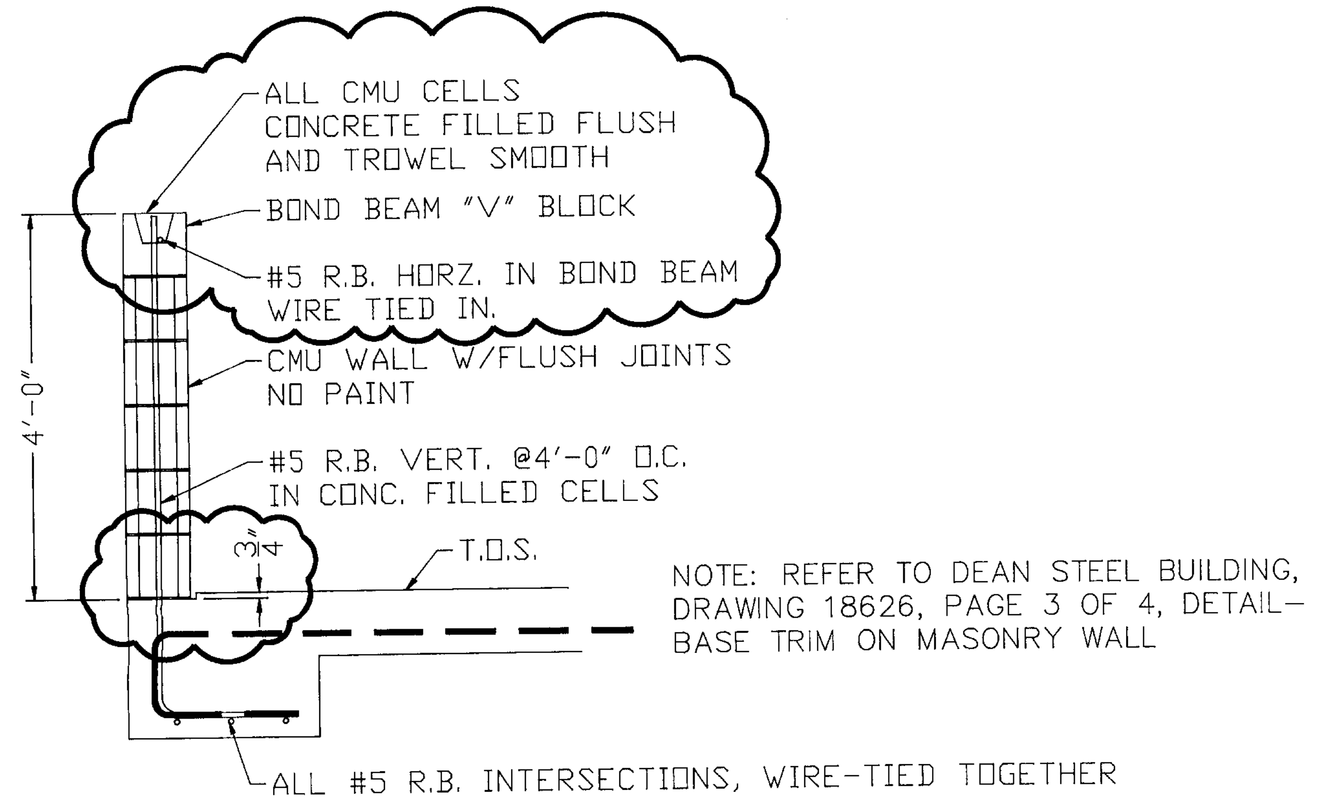
SECTION C-C CONCRETE MASONRY UNIT (CMU) 1" = 1'-0"
