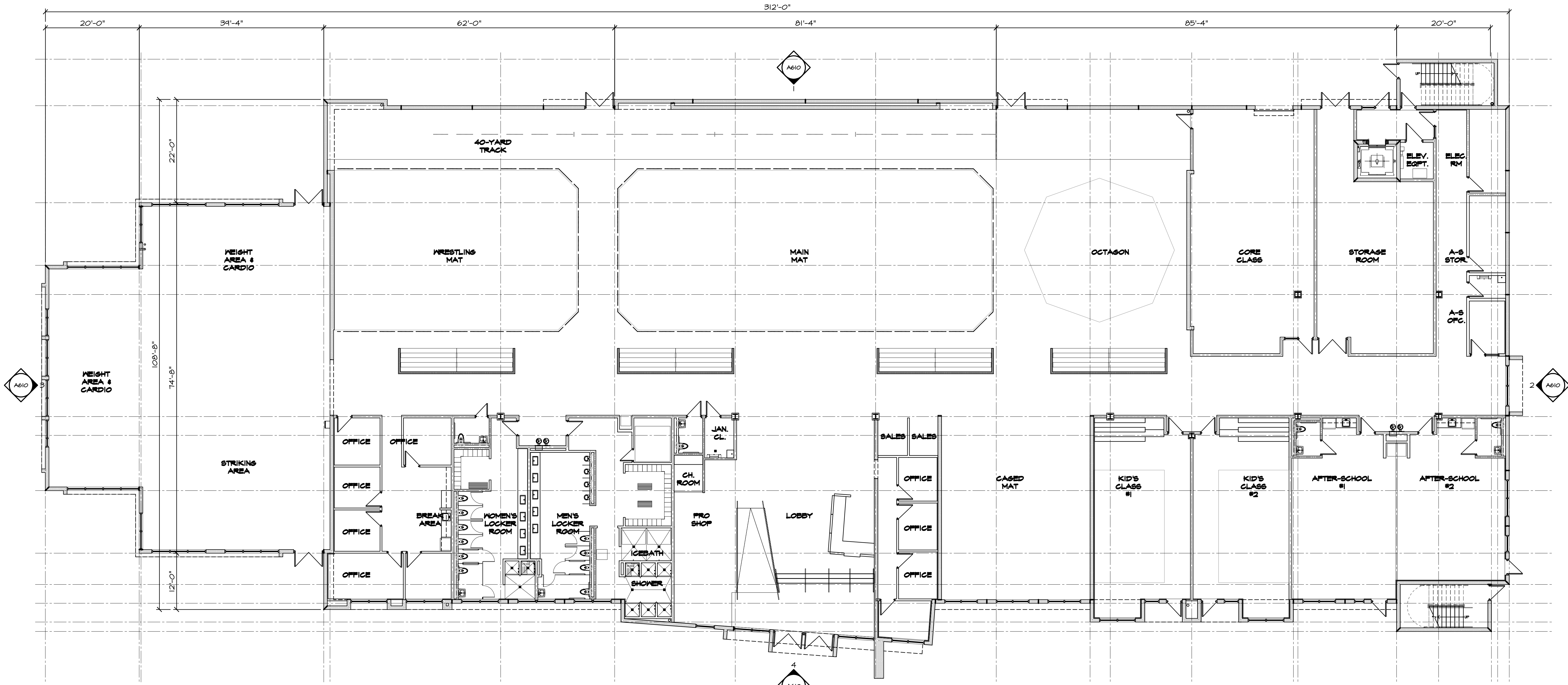
FIRST FLOOR PLAN 3/32" = 1'-0"
