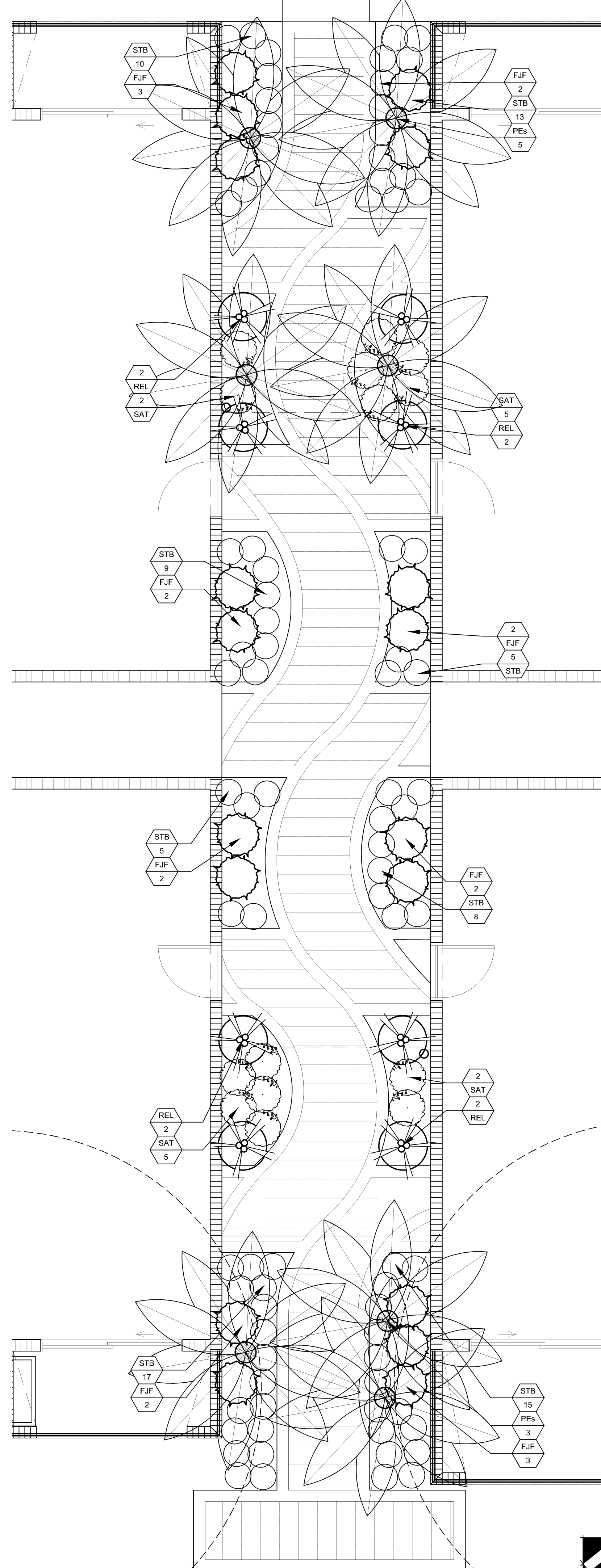
BUILDING 11 COURTYARD LANDSCAPE PLAN SCALE: 1/4" = 1'-0"
