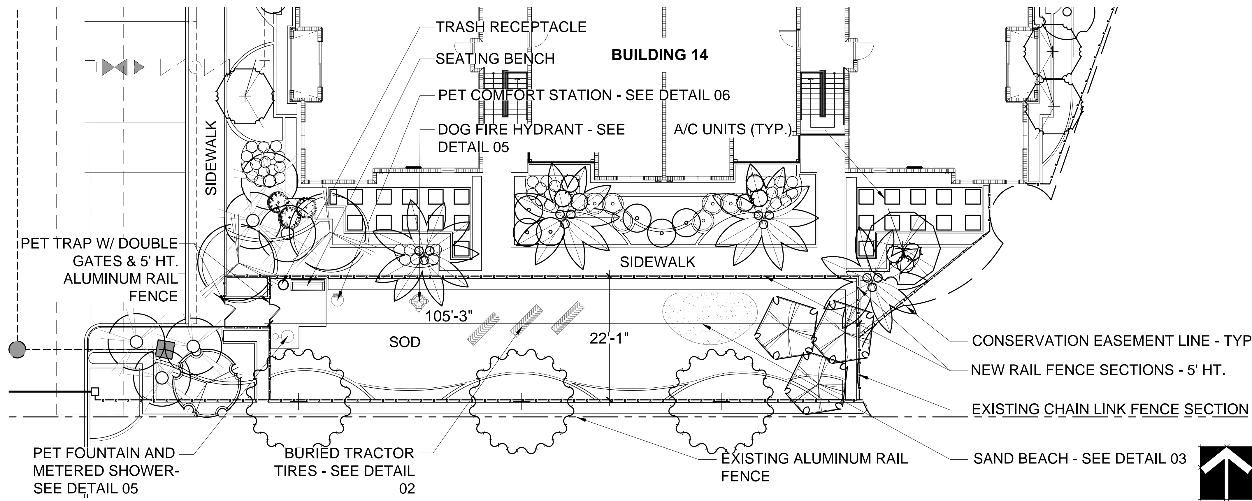
01 DOG PARK ENLARGED PLAN
