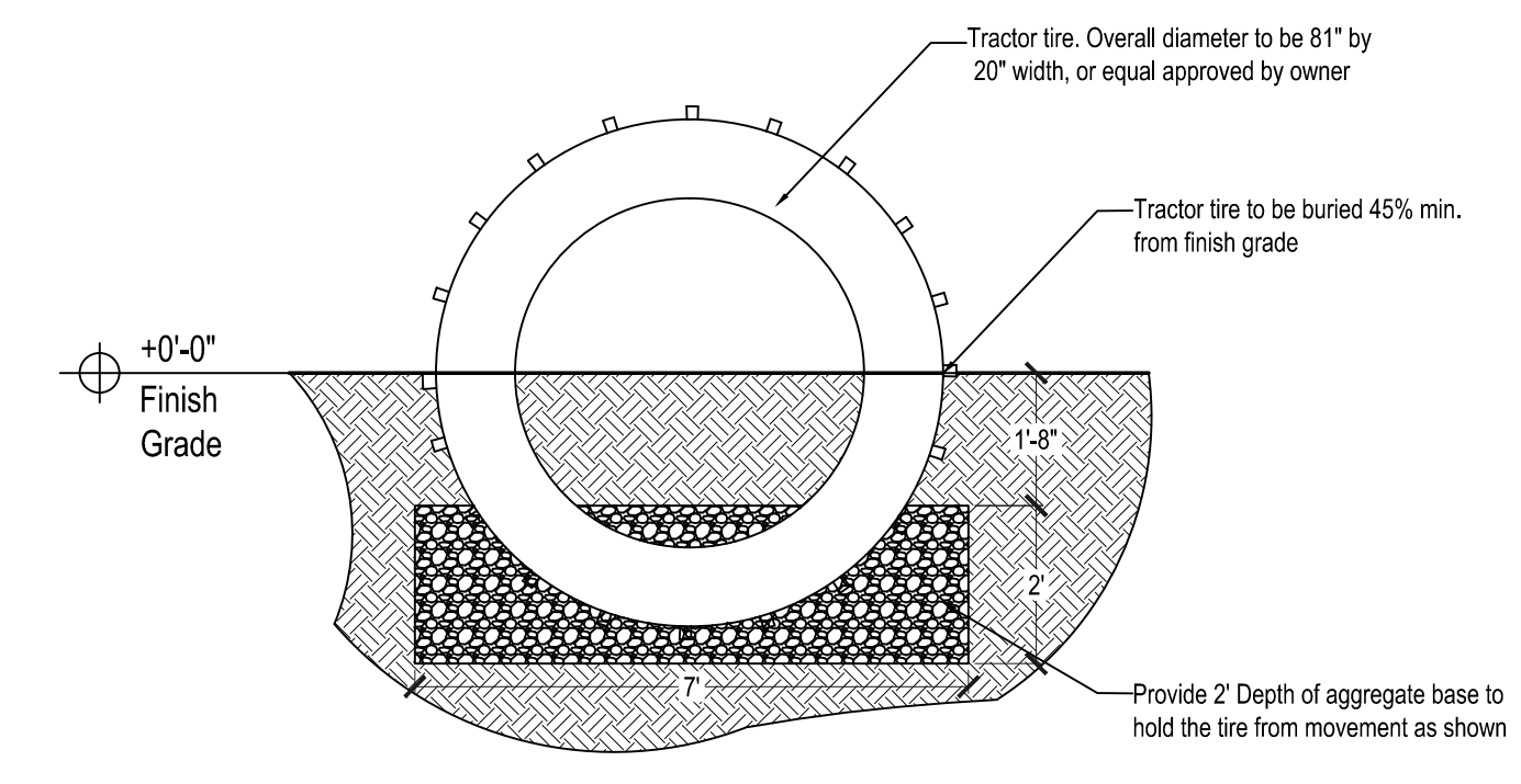
02 BURIED TRACTOR TIRE DETAIL
