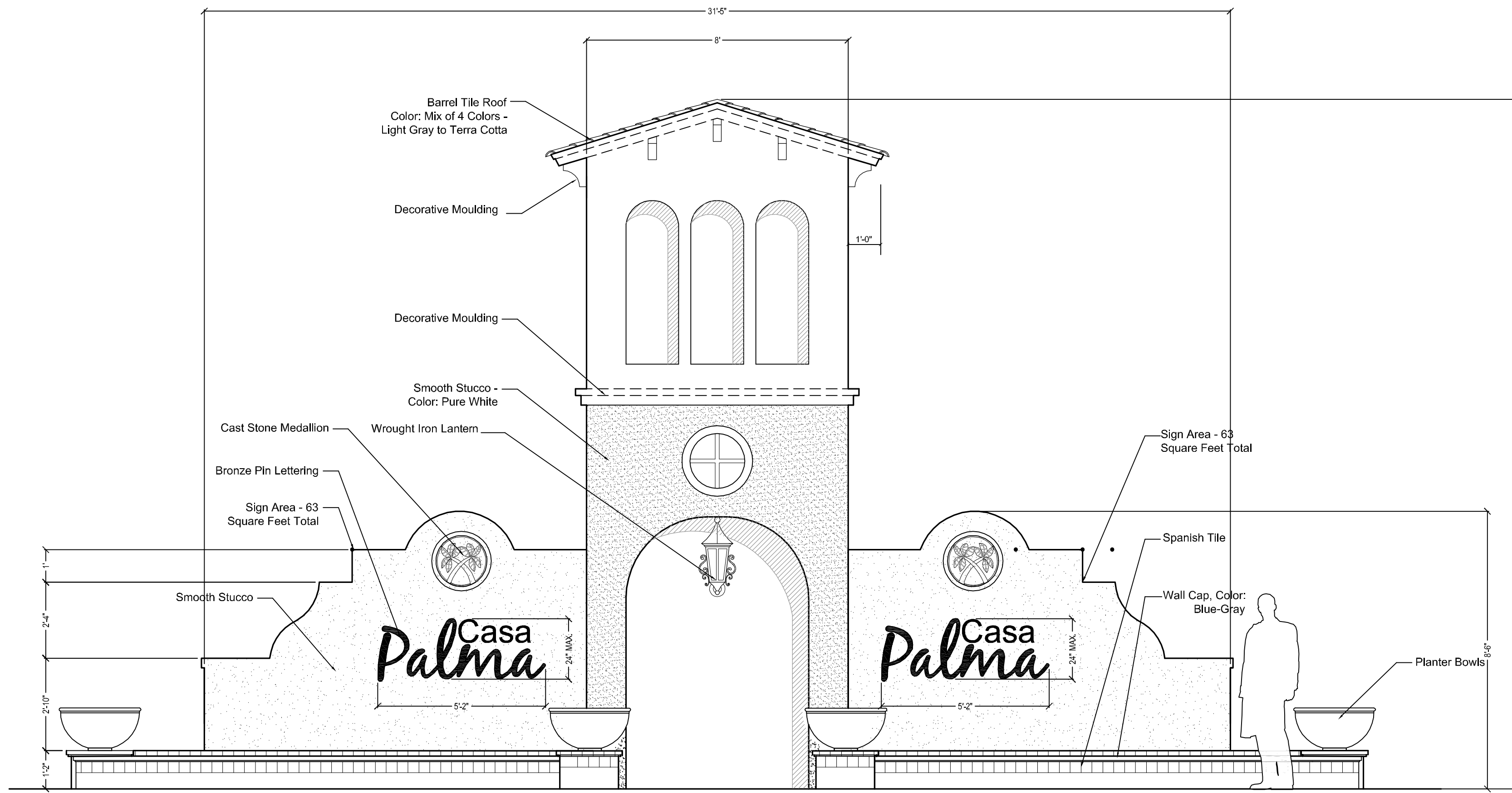
01 MONUMENT SIGN ELEVATION
