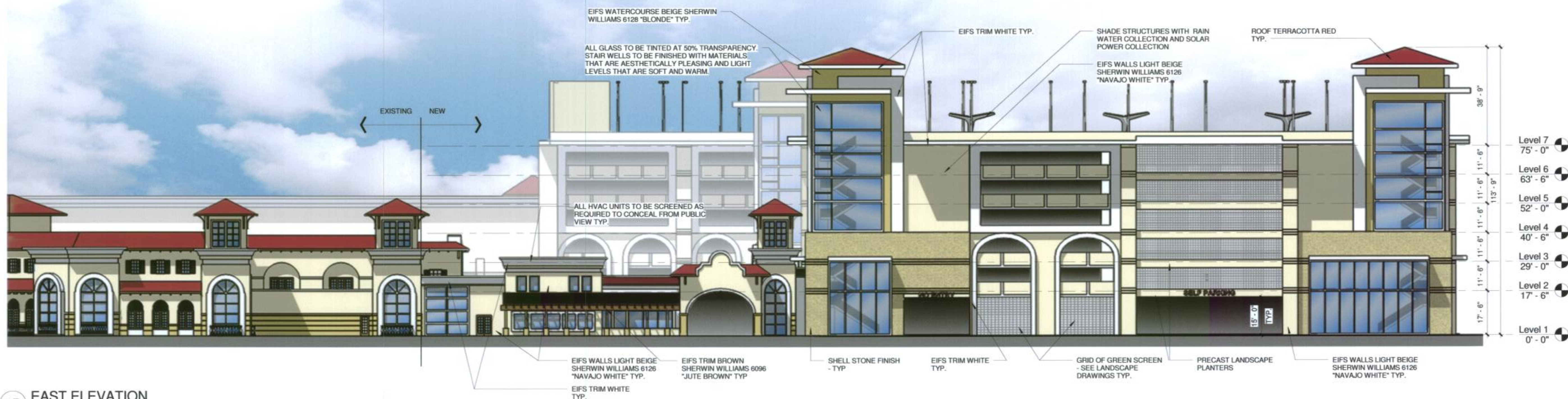
1B EAST ELEVATION 3/64" = 1'-0"
