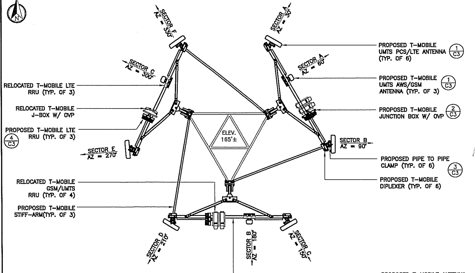
EXISTING ANTENNA MOUNT DETAIL
