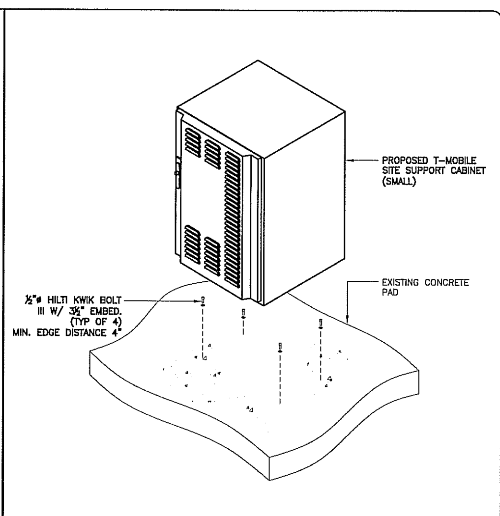
SSC CABINET CONNECTION DETAIL NTS 3
