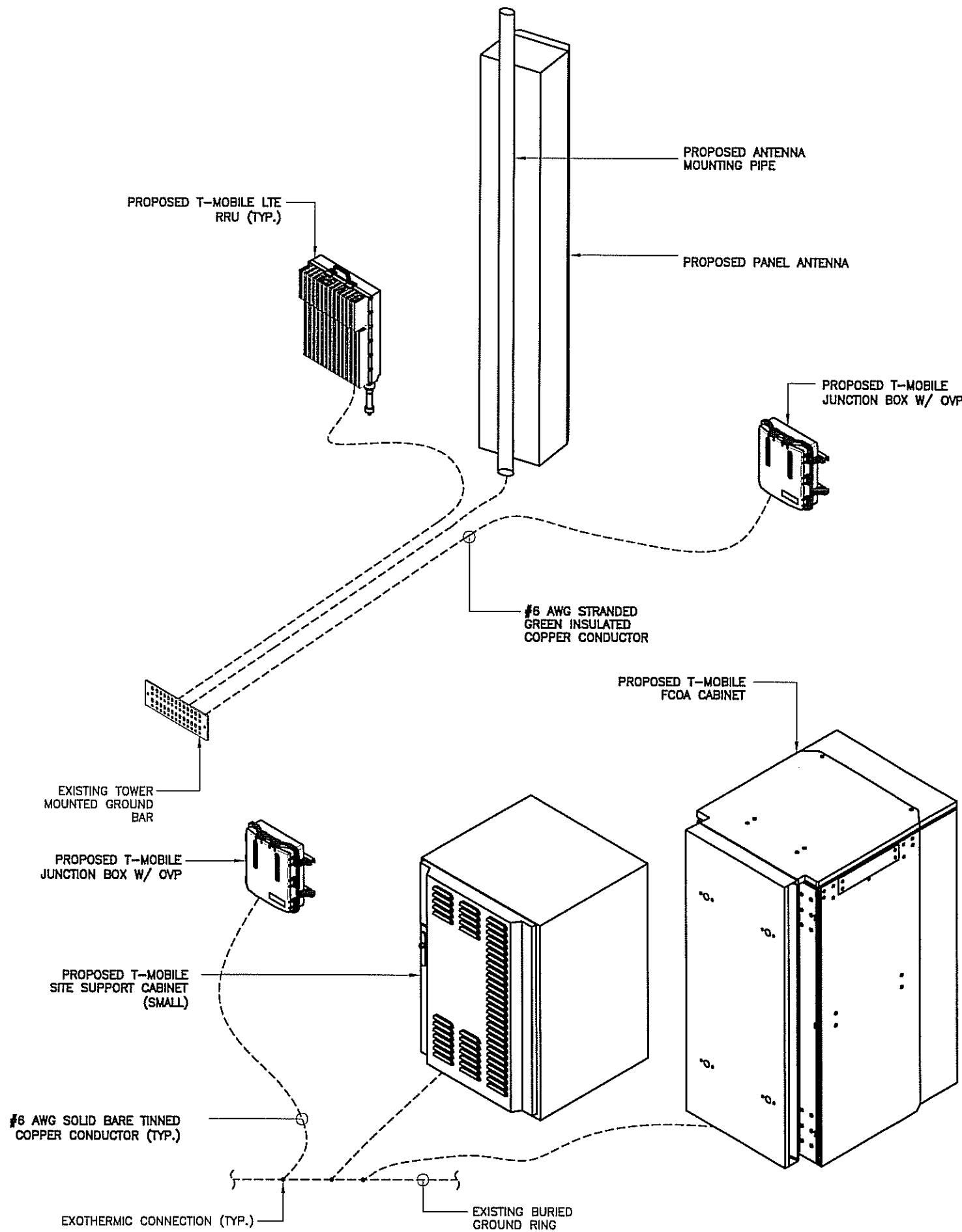
GROUNDING DIAGRAM (TYP.)
