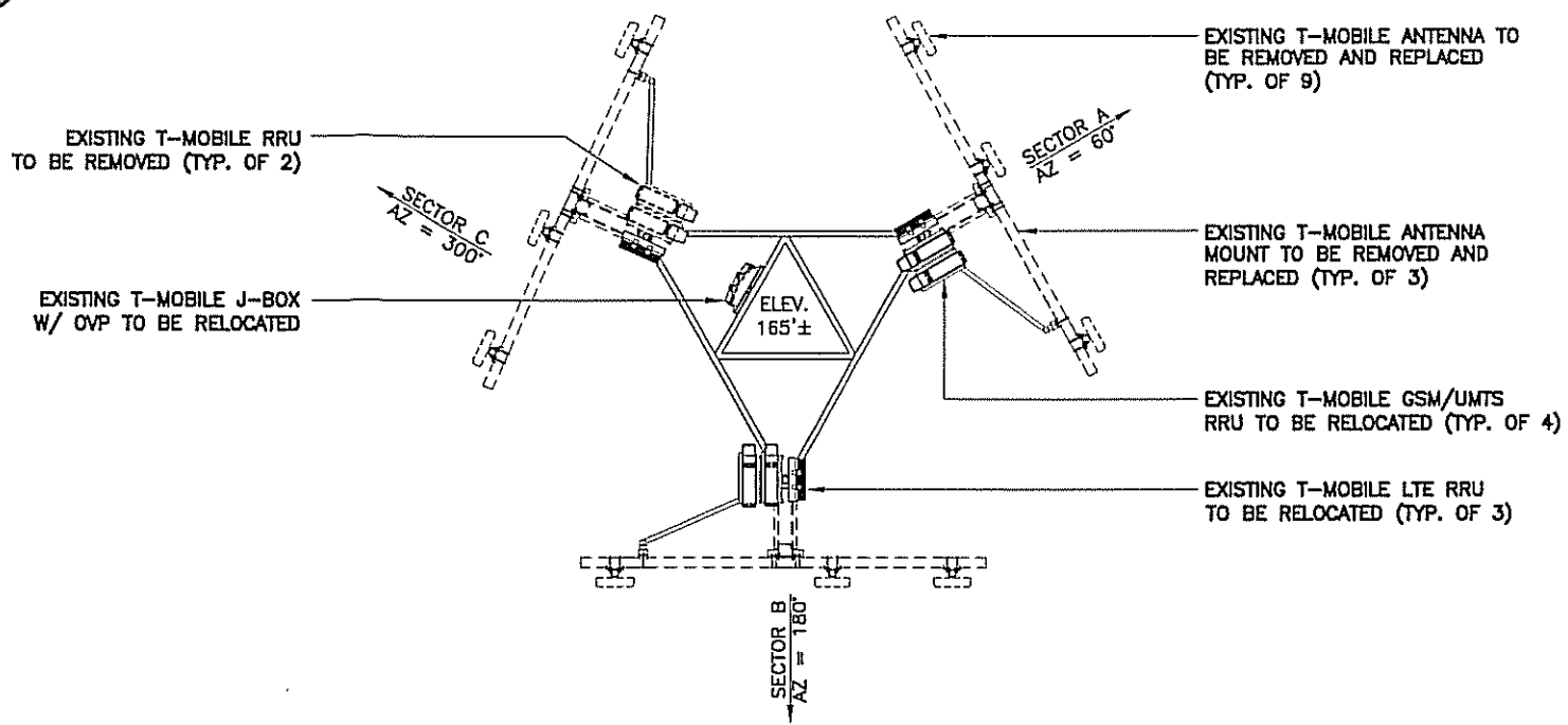
EXISTING ANTENNA MOUNT DETAIL
