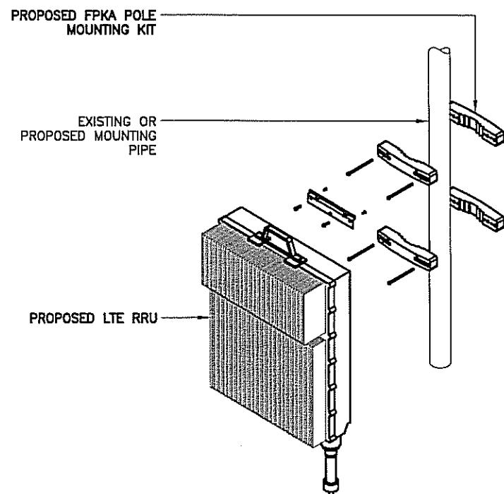
LTE RRU MOUNTING DETAIL
