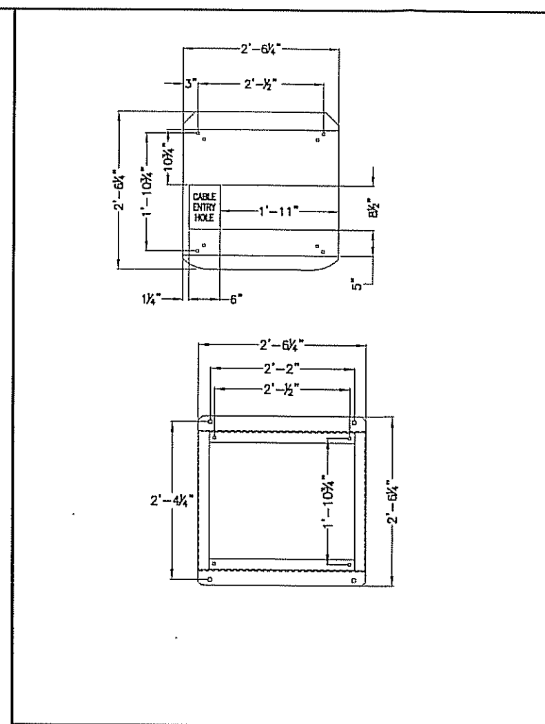
FCOA CABINET MOUNTING FOOTPRINT NTS 2
