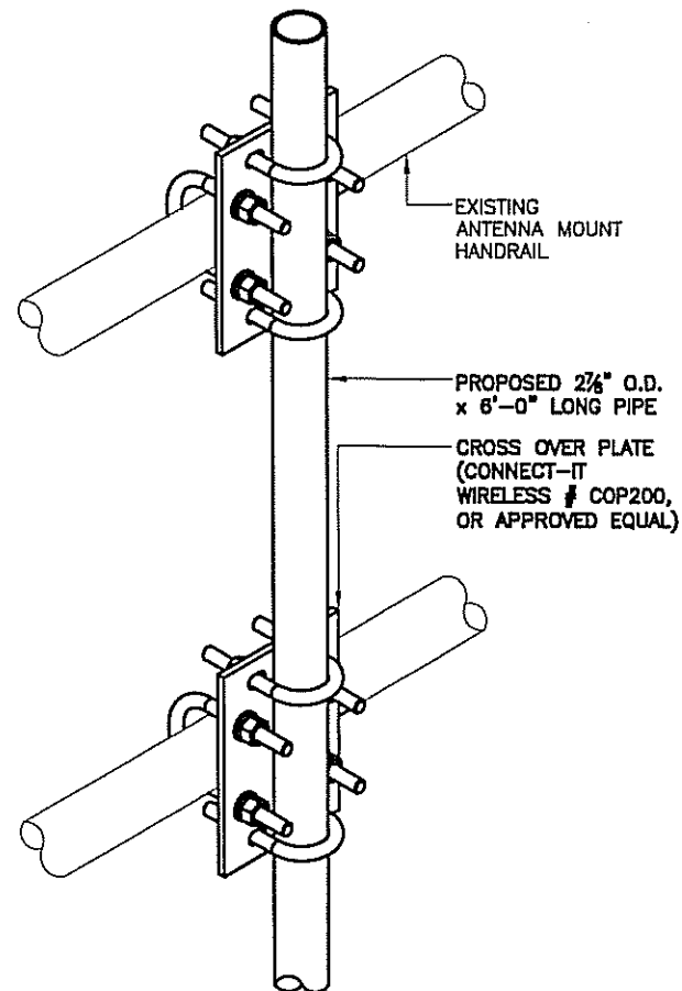
PIPE MOUNTING DETAIL
