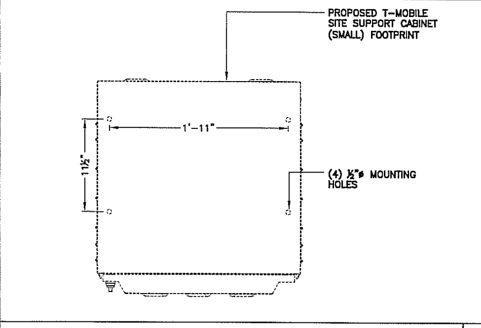
SSC CABINET MOUNTING FOOTPRINT NTS 4
