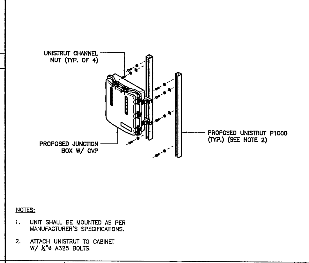
J-BOX W/ OVP MOUNTING DETAIL NTS 5
