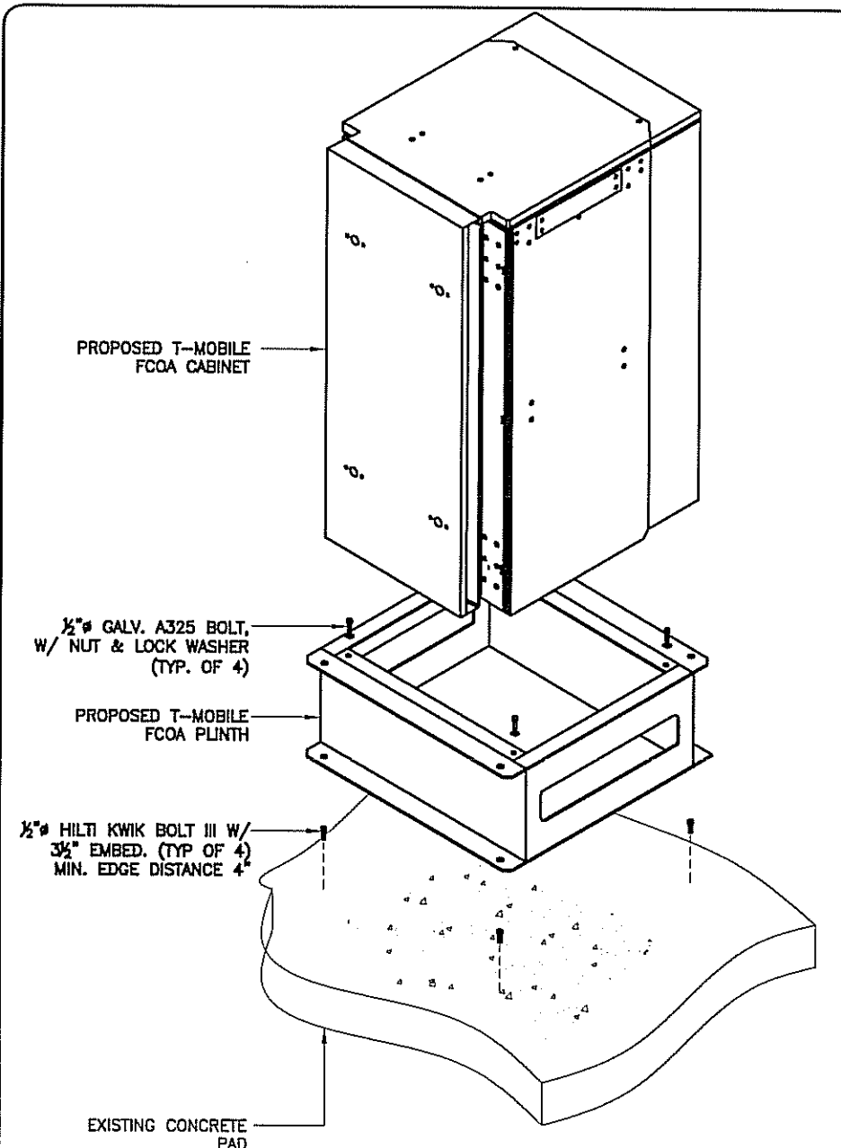
FCOA CABINET CONNECTION DETAIL NTS 1
