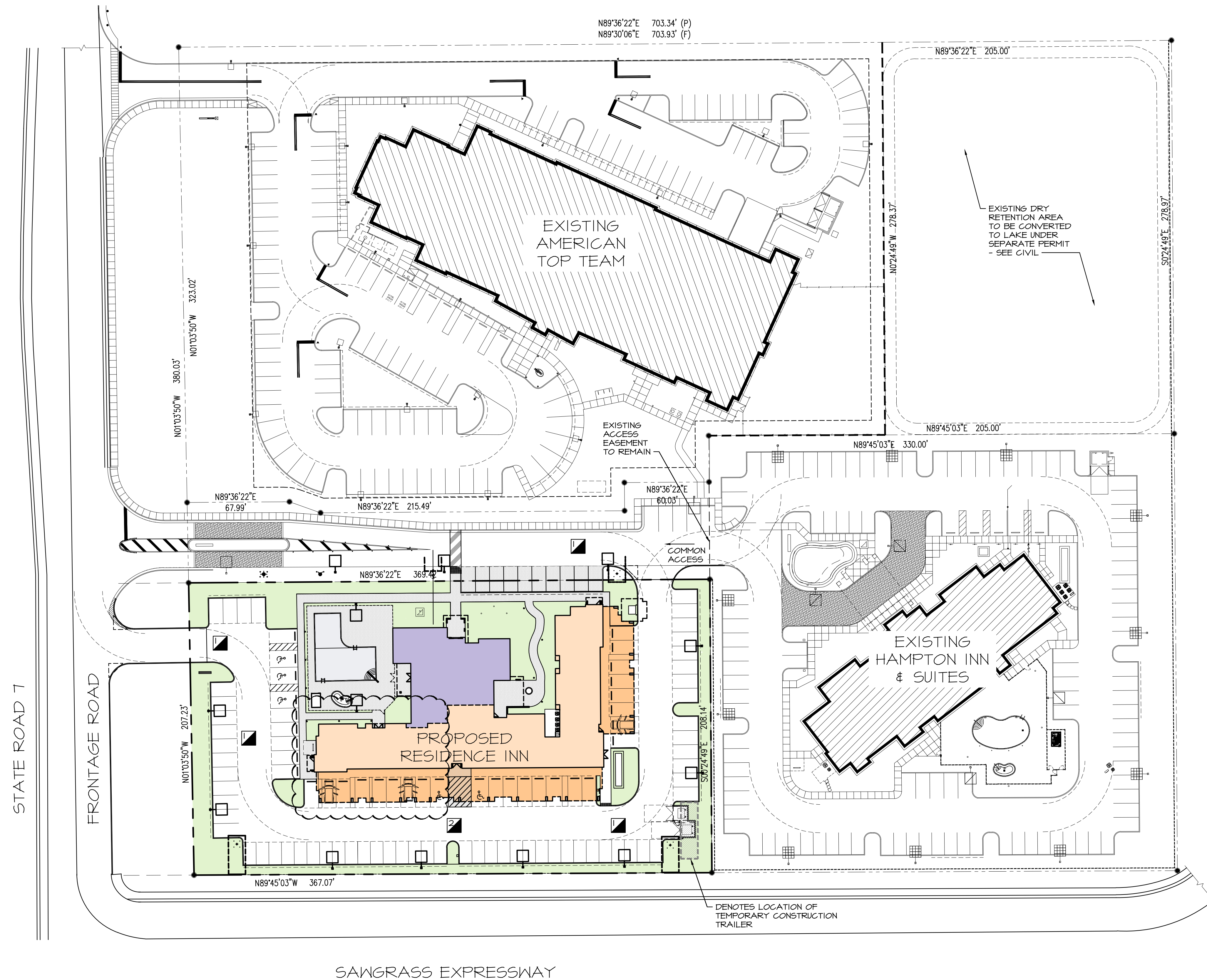
OVERALL SITE PLAN 1"=40'-0"
