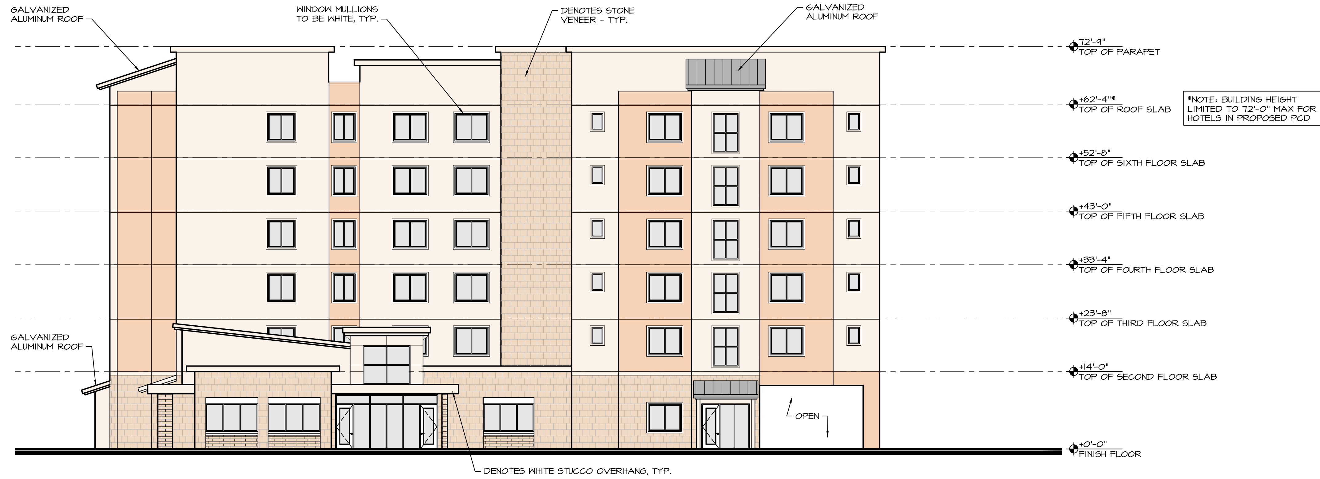
WEST ELEVATION
