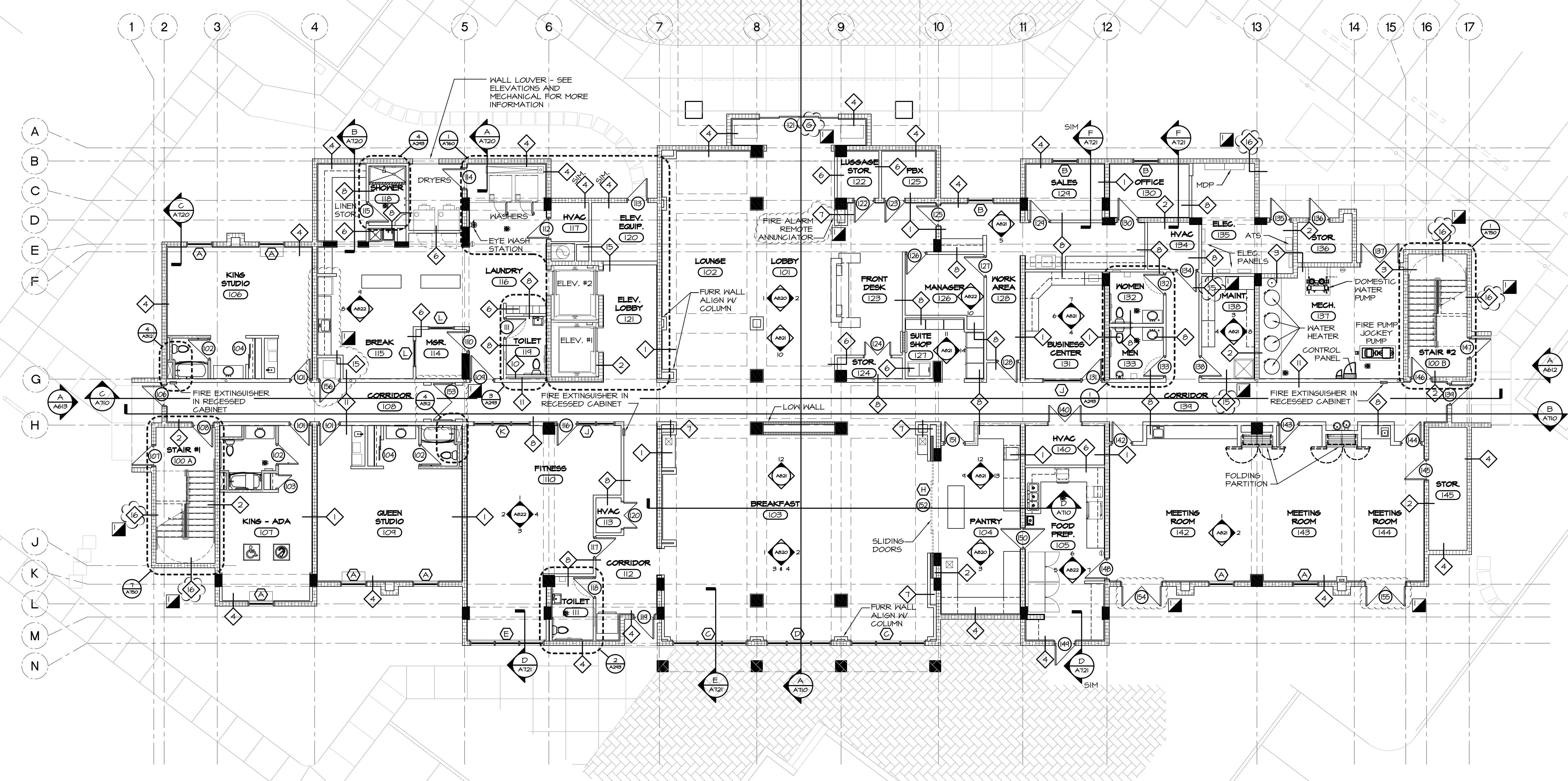
FIRST FLOOR PLAN 1/8"=1'-0"
