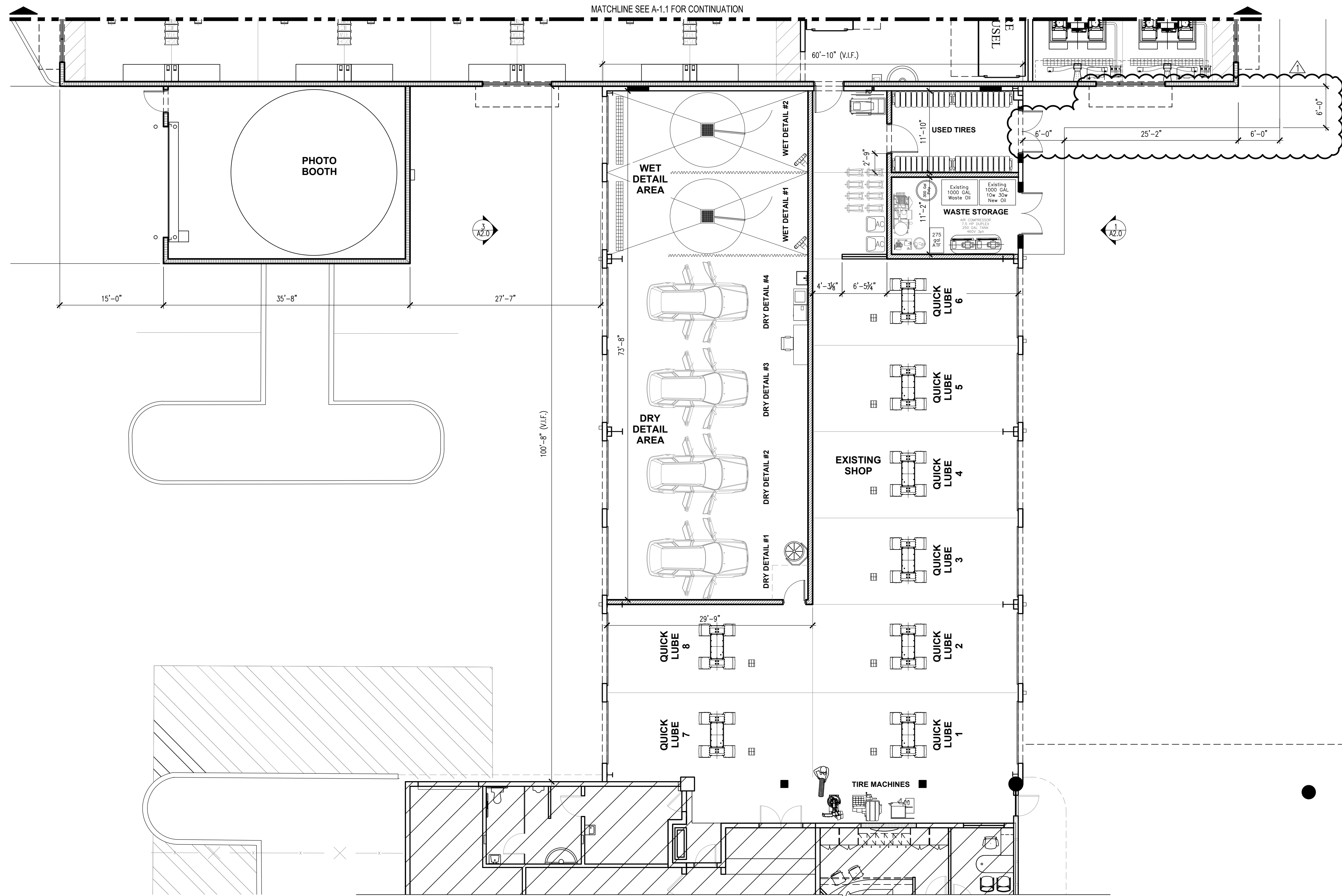
2 ENLARGED PLAN - PHOTO BOOTH AND EXISTING SHOP RENOVATION SCALE: 1/8"=1'-0"
