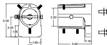
MAF - HORIZONTAL MAST ARM FITTER
