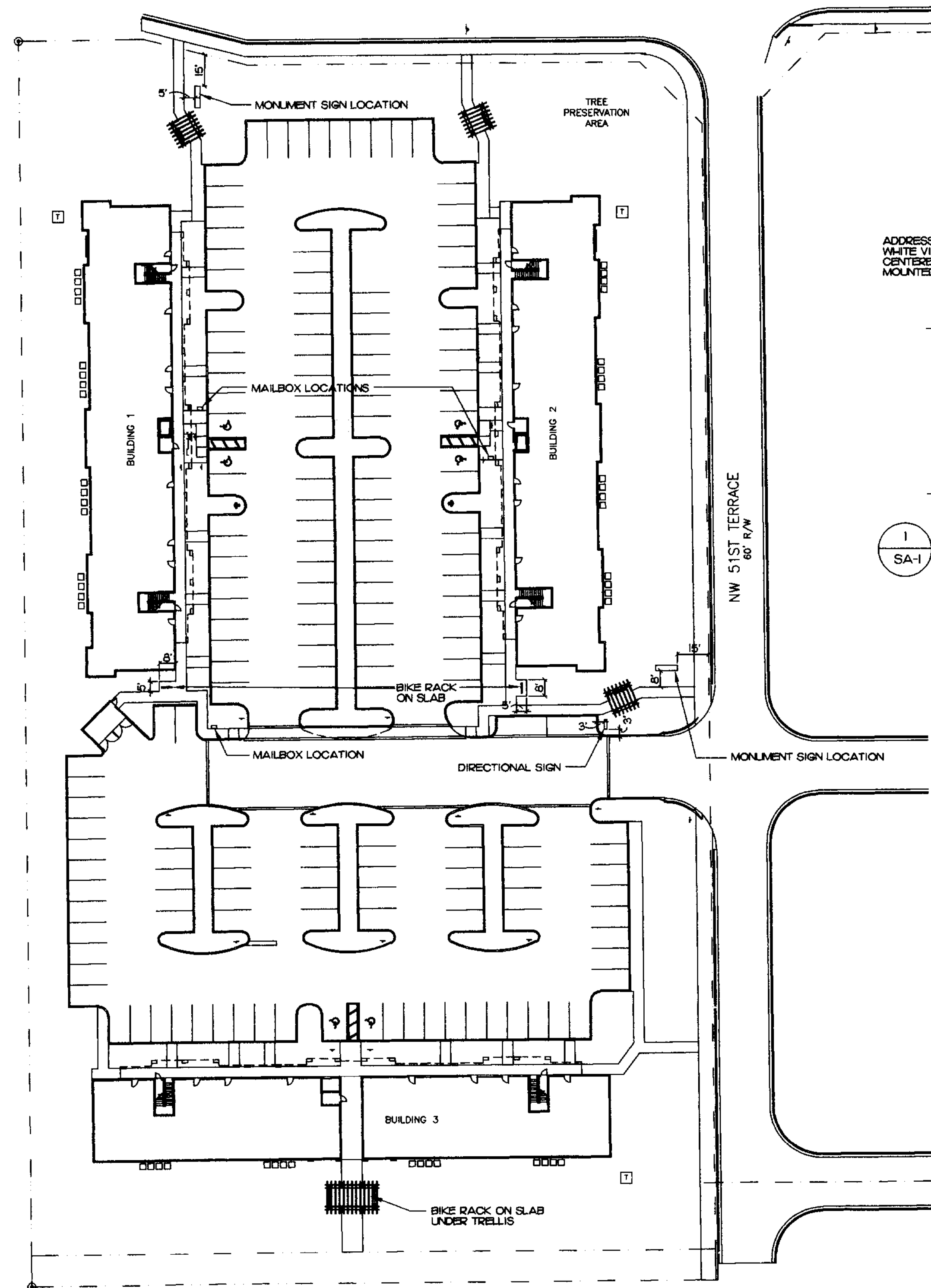
UNIFORM MASTER SIGN PLAN SCALE: 1" = 40'-0"
