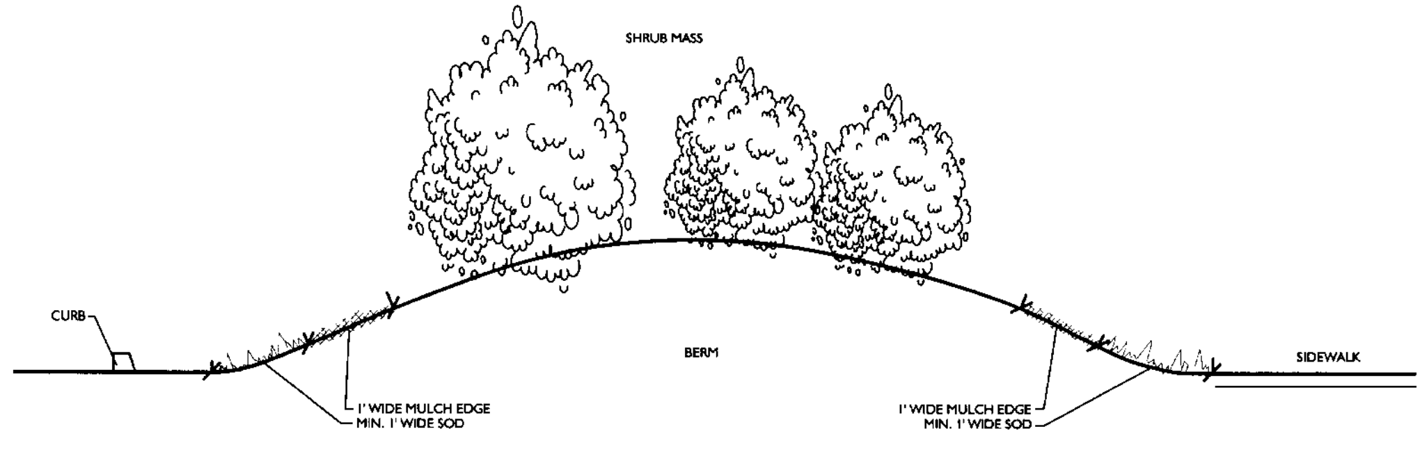
TYPICAL BUFFER EDGE SECTION NTS
