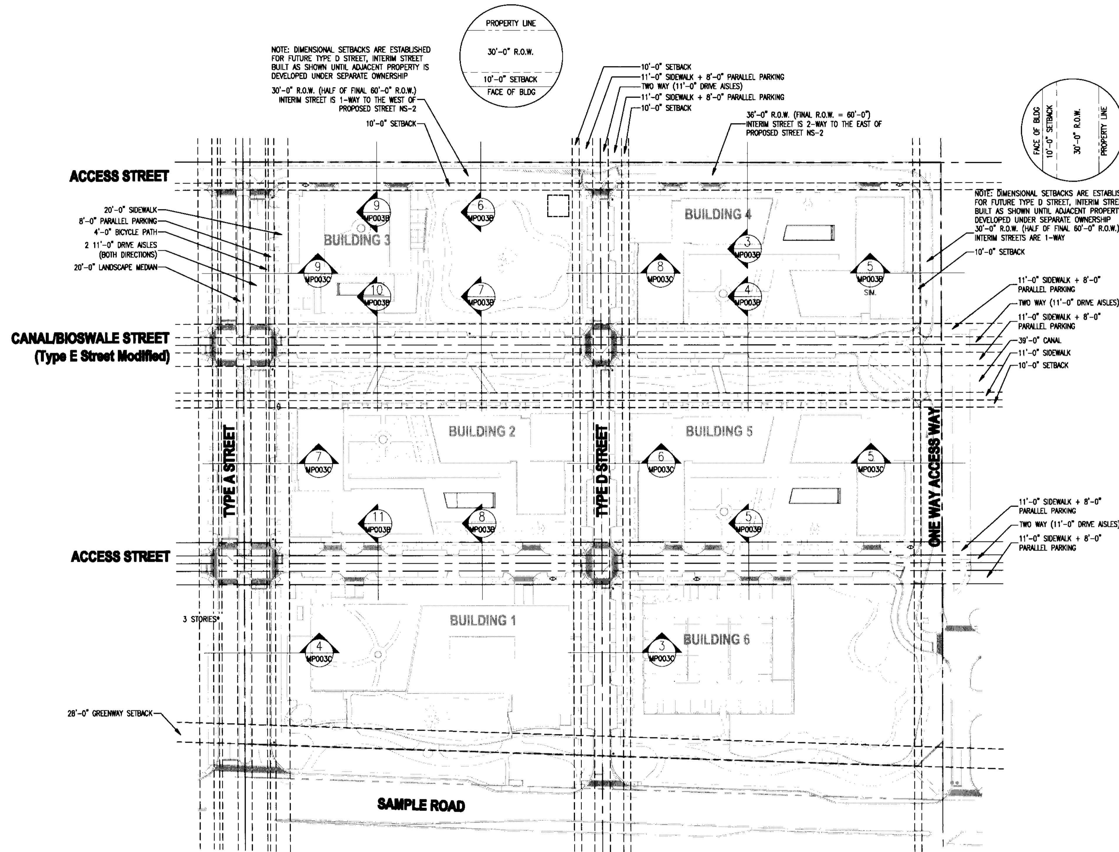
1 OVERALL RIGHT OF WAY PLAN OPTION A SCALE: 1" = 80'-0"
