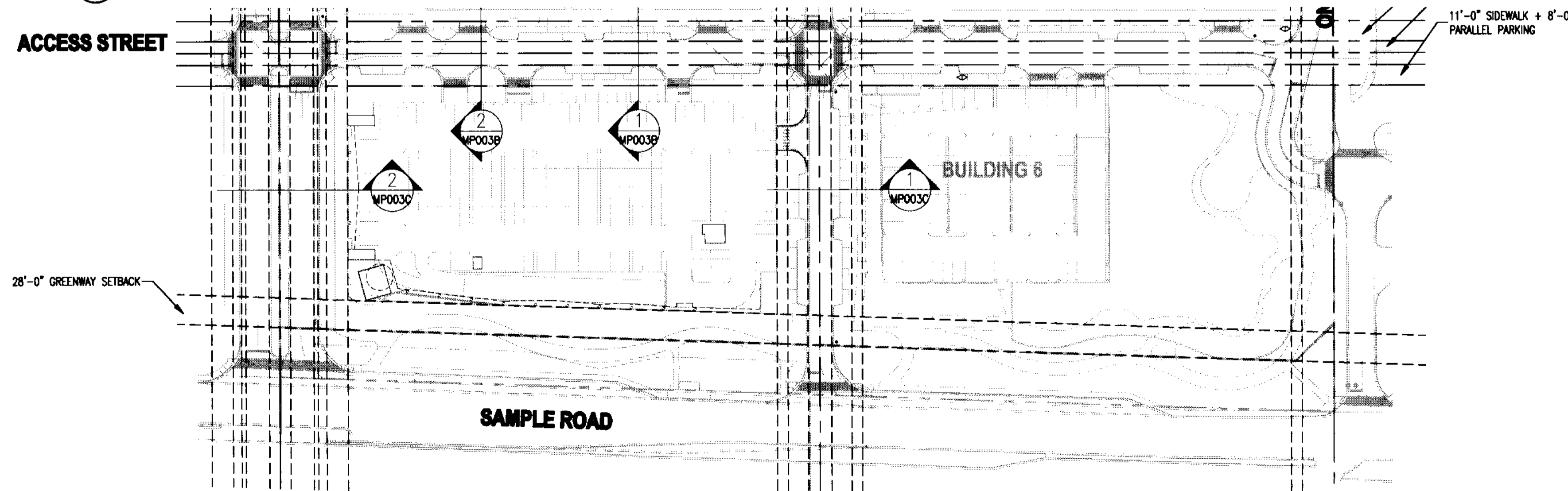
2 OVERALL RIGHT OF WAY PLAN OPTION B SCALE: 1" = 80'-0"
