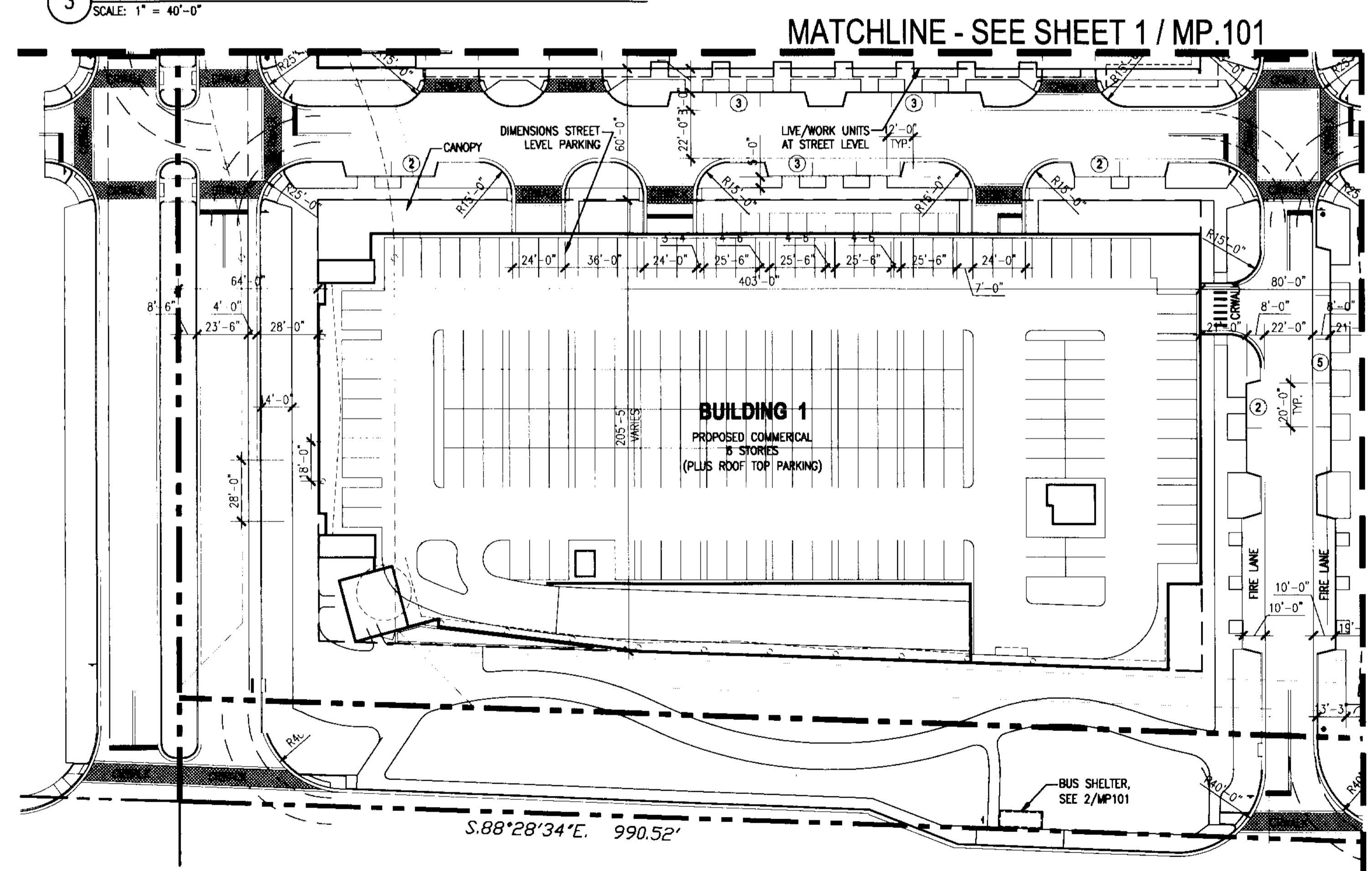
2 PARTIAL ENLARGED GEOMETRIC CONTROL PLAN - DEALERSHIP OPTION B SCALE: 1" = 40'-0"
