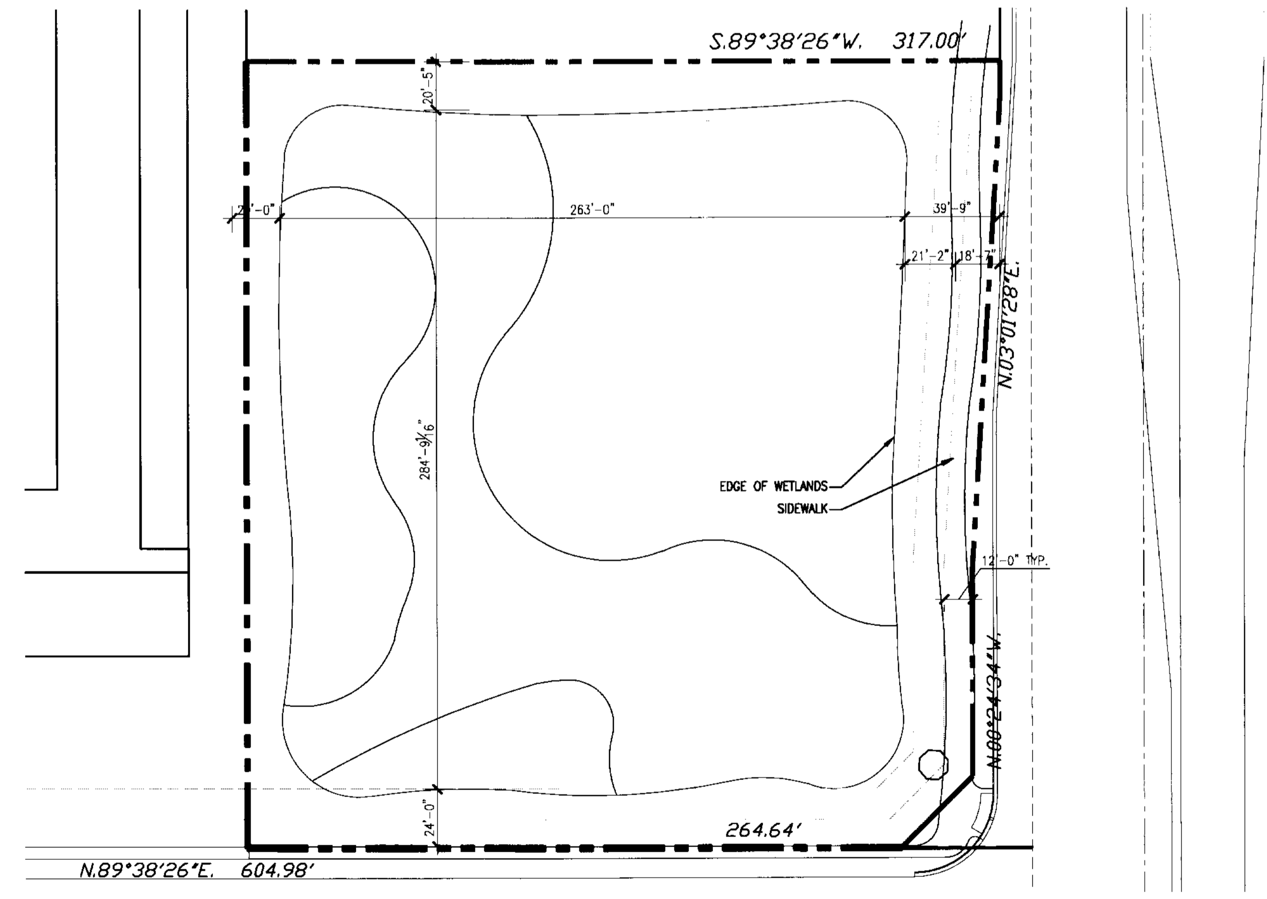
1 PARTIAL ENLARGED GEOMETRIC CONTROL PLAN SCALE: 1" = 40'-0"
