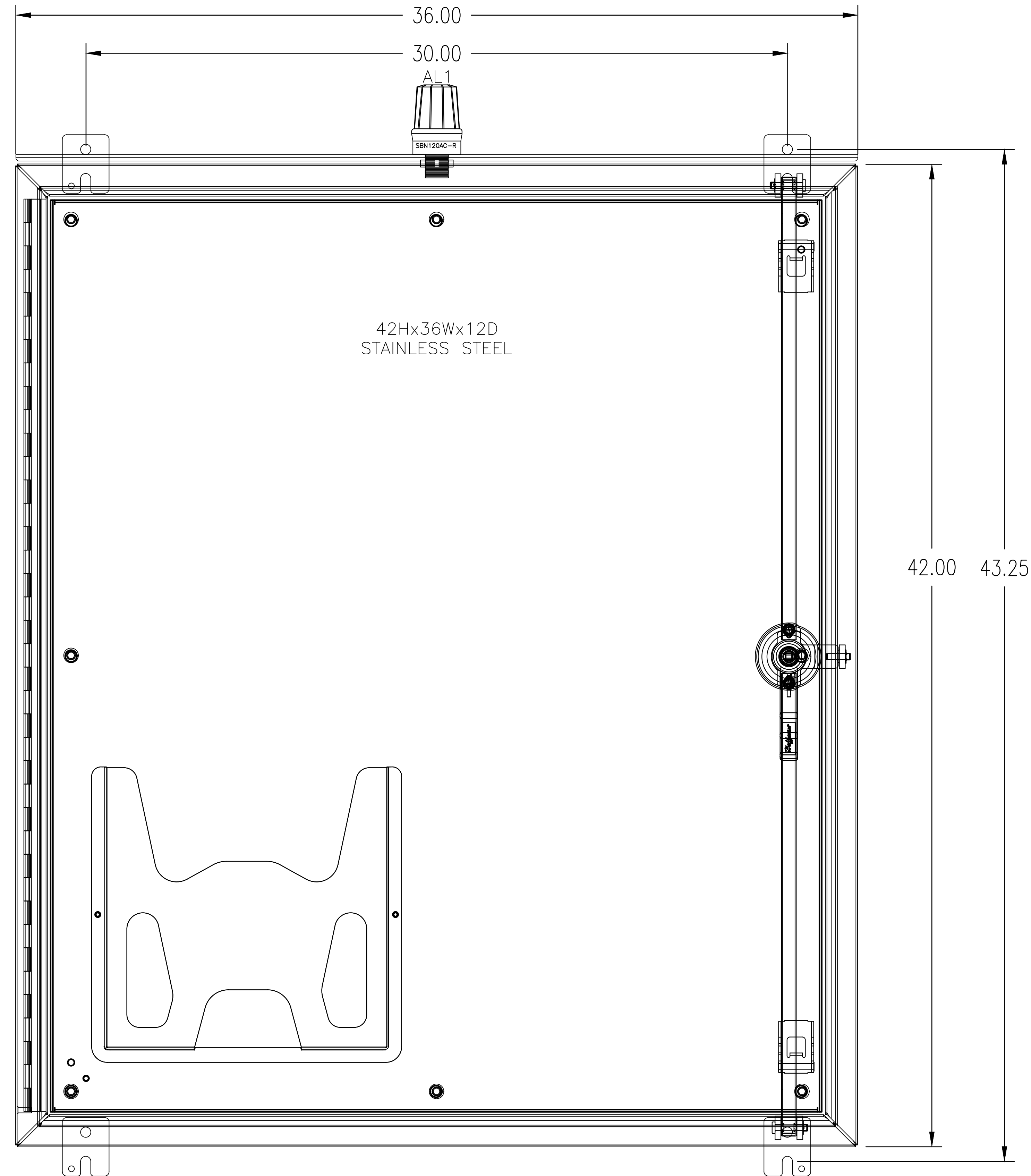
FRONT VIEW
