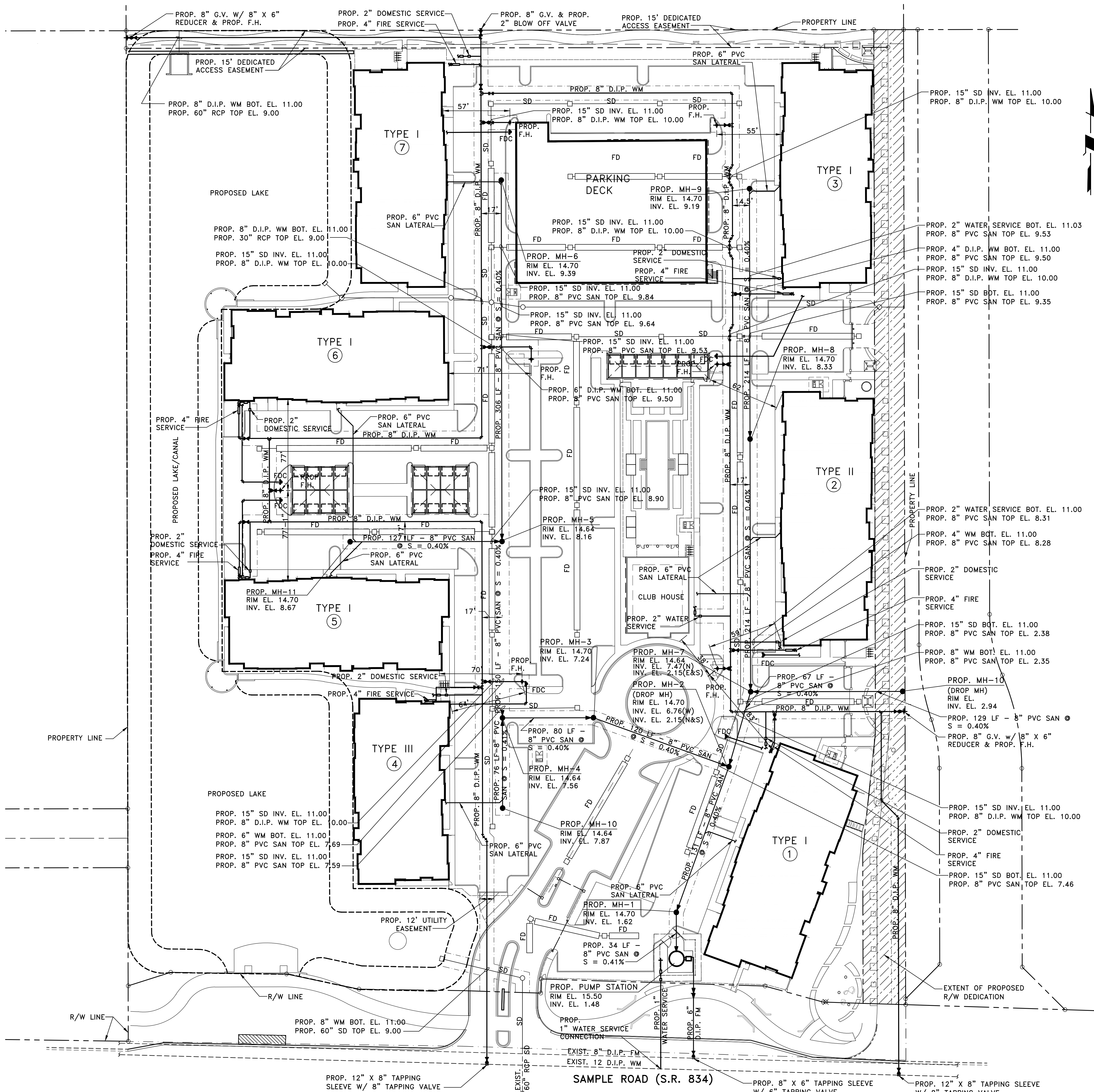
WATER AND SEWER PLAN SCALE: 1" = 40'
