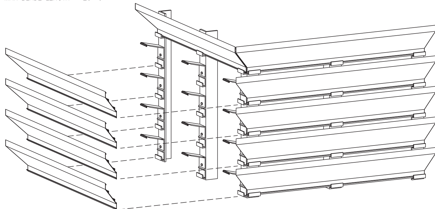
ARCHITECTURAL ROOF SCREEN TYPICAL CONSTRUCTION
