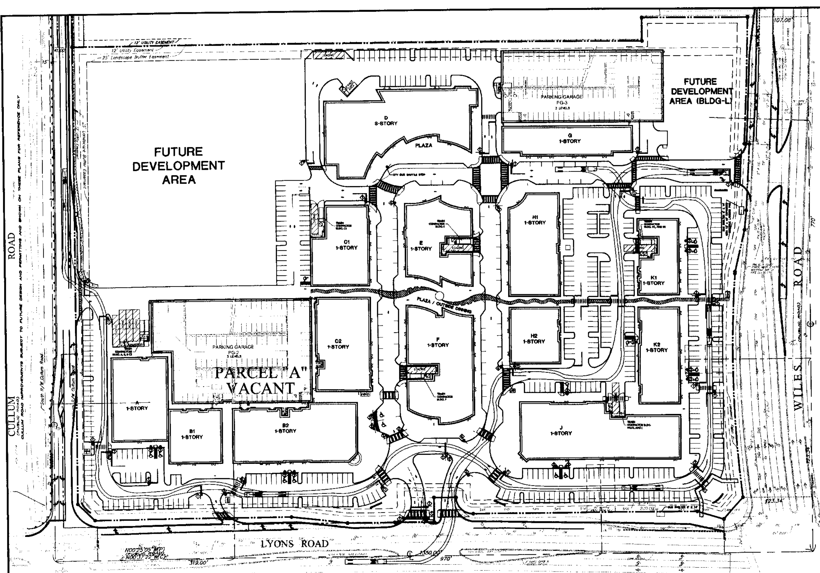
VIEW A FIRE TRUCK
