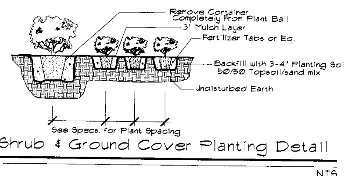
LPI0 D PLANTING DETAIL TYP.
