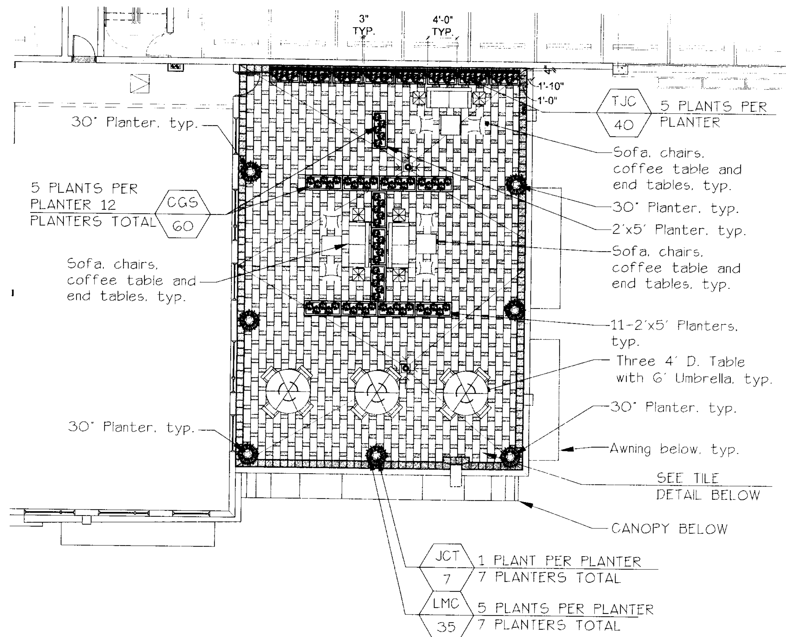
LPI0 A BUILDING 'G' TERRACE LANDSCAPE PLANTER PLAN SCALE: 1/8" = 1'-0"
