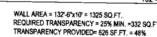
7 112 TYP. WALL FENESTRATION BUILDING E. F. J 1" = 20'
