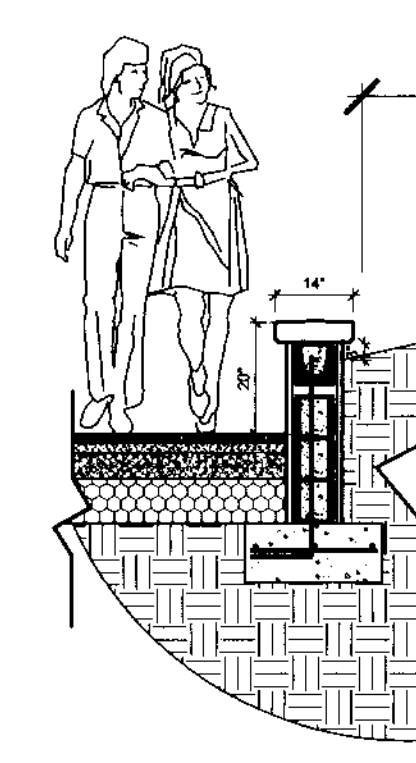
8/1/08 ENLARGEMENT OF SEAT WALL PLANTER FILL, TYP.
