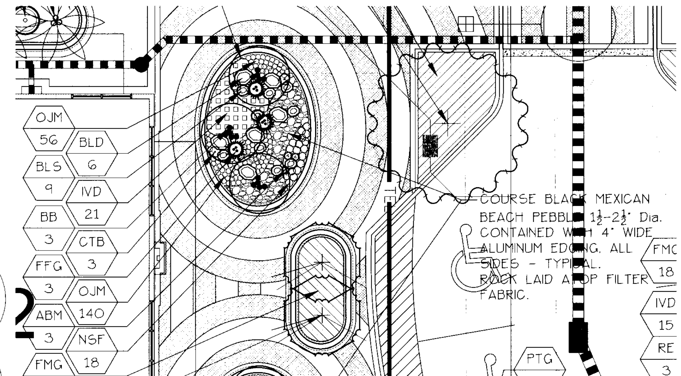
ENLARGEMENT OF OVAL SEAT WALL PLANTER, TYP.
