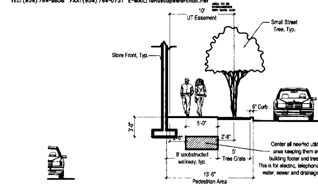
OO1 SECTION OF TREE TO BUILDING IN RELATION TO UNDERGROUND UTILITIES. TYP.
