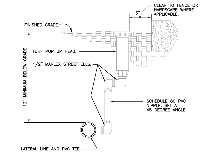
6 TURF SPRAY MARLEX ASSEMBLY 3" = 1'-0" FX-IR-FX-BACK-03
