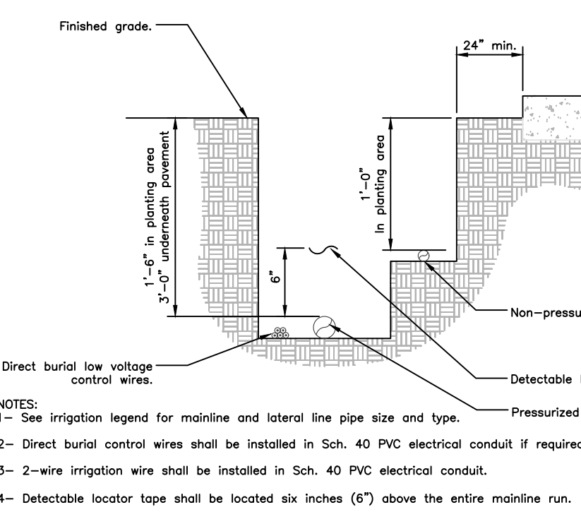
5 IRRIGATION TRENCHING 1 1/2" = 1'-0" FX-IR-FX-BACK-03
