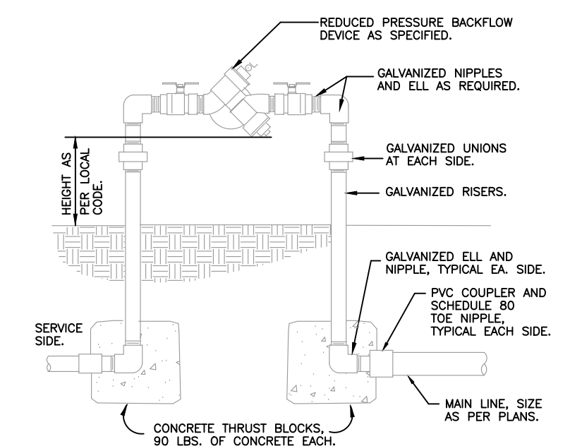
3 REDUCED PRESSURE BACKFLOW DEVICE 1" = 1'-0" FX-IR-FX-BACK-03
