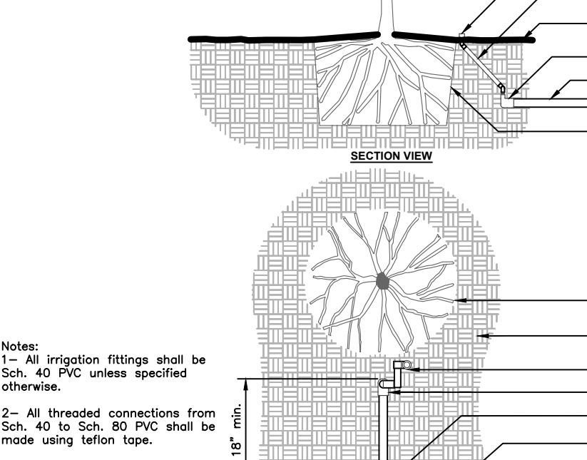
9 IRRIGATION BUBBLER W/ LAYOUT 3/4" = 1'-0" FX-IR-FX-BACK-03
