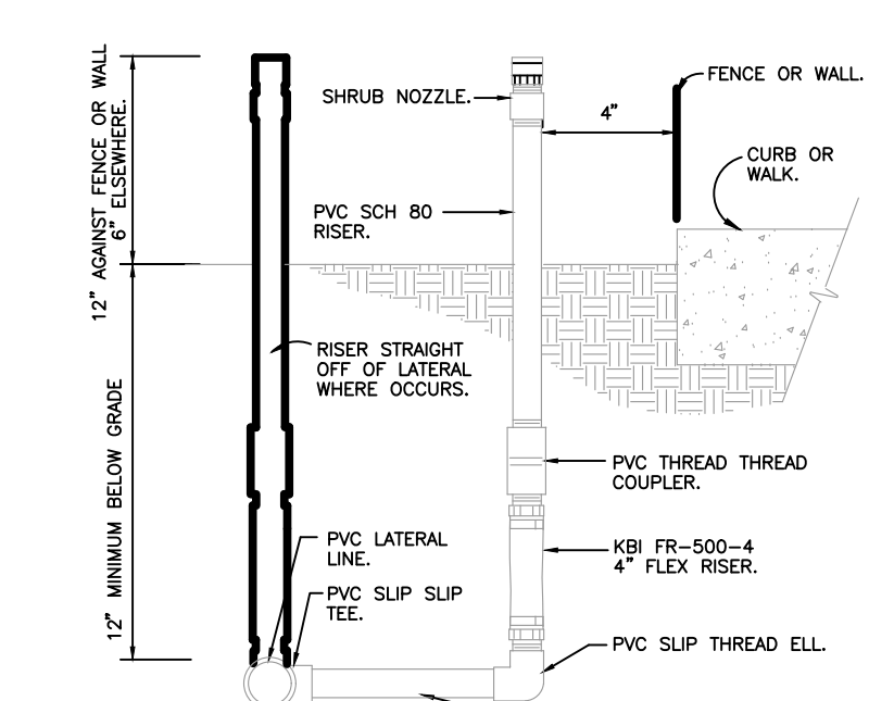
7 SHRUB SPRAY KBI FIXED RISER 3" = 1'-0" FX-IR-FX-HEAD-07
