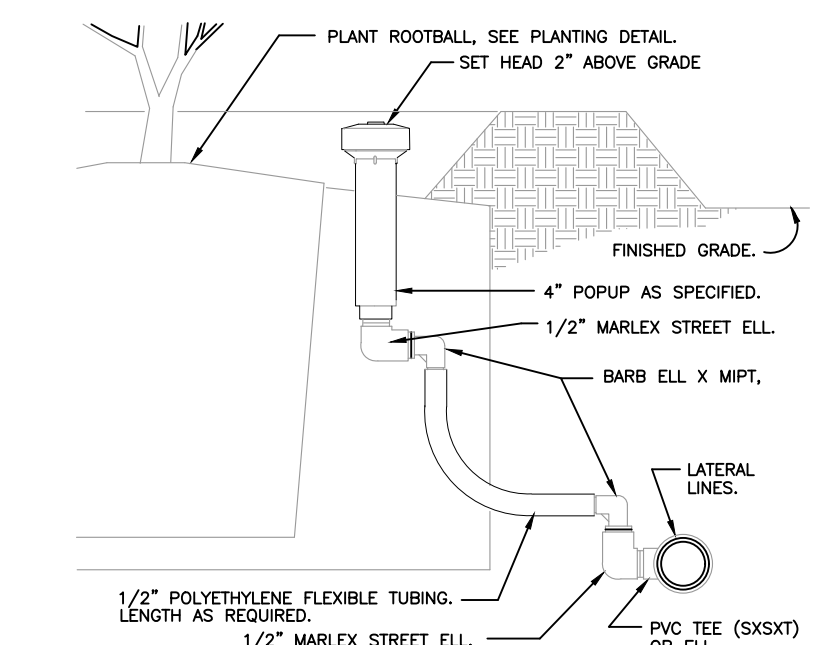
8 POPUP BUBBLER 3" = 1'-0" FX-IR-FX-BACK-03
