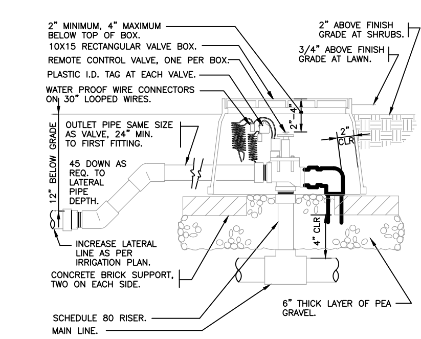
2 ELECTRIC REMOTE CONTROL VALVE 1 1/2" = 1'-0" FX-IR-FX-BACK-03
