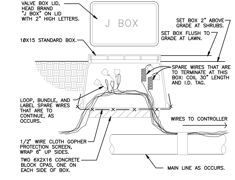
4 WIRE BUNDLE JUNCTION BOX 1 1/2" = 1'-0" FX-IR-FX-BACK-03
