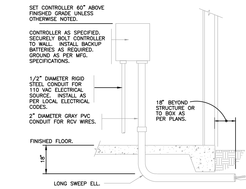
1 INTERIOR WALL MOUNT CONTROLLER 1" = 1'-0" FX-IR-FX-CONT-14
