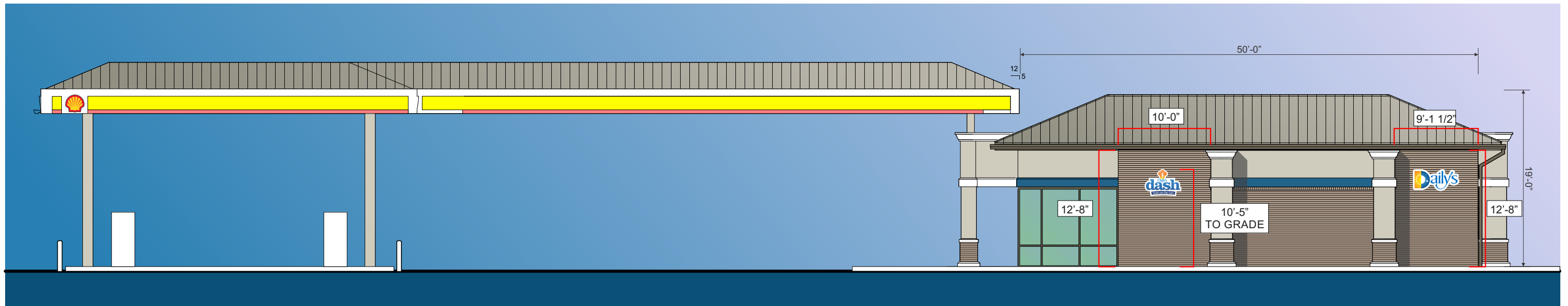
South Elevation - Illuminated Contour Cabinet Sign 3/32" = 1'-0"
