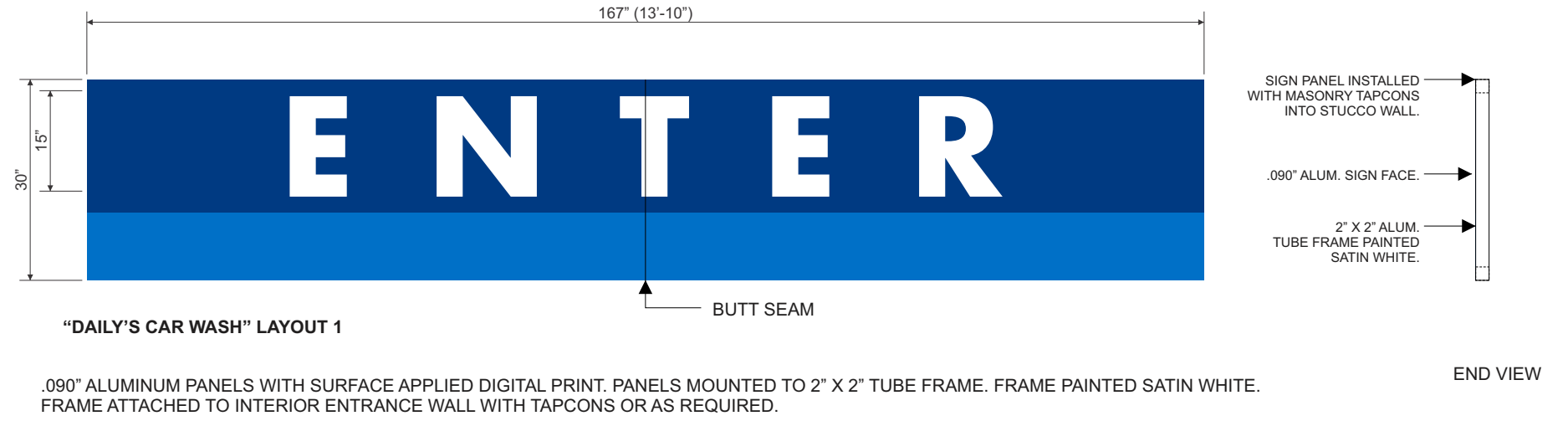
G.1 Front Elevation - Single Sided Entrance Sign 1/2" = 1'-0"
