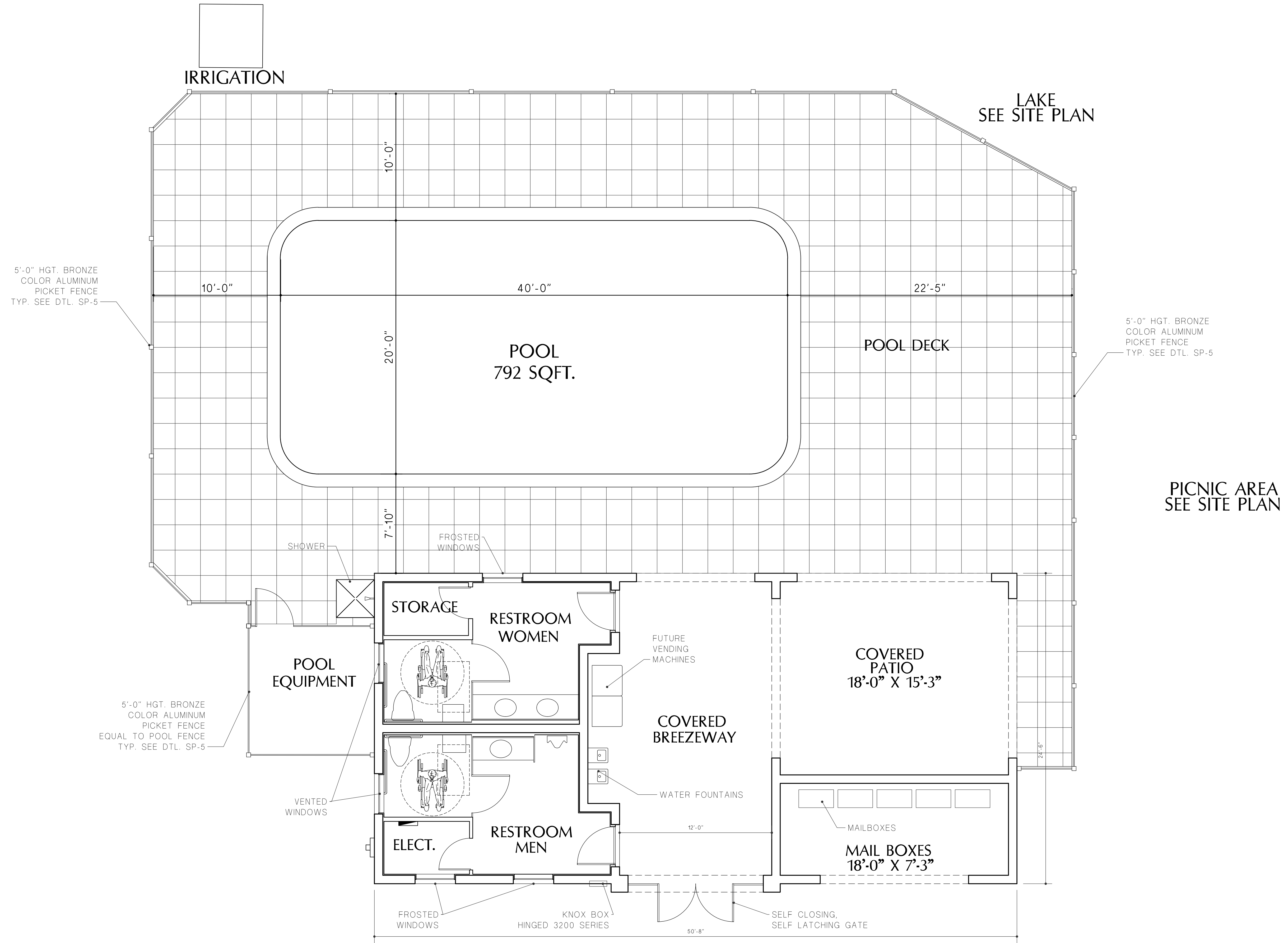
POOL PAVILION FLOOR PLAN SCALE: 1/4" = 1'-0"
