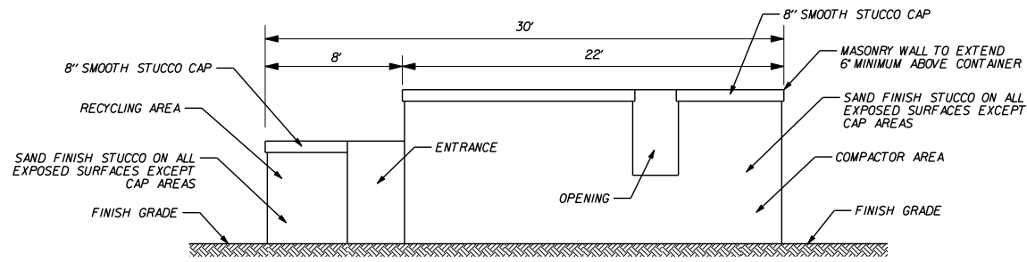
SIDE ELEVATION
