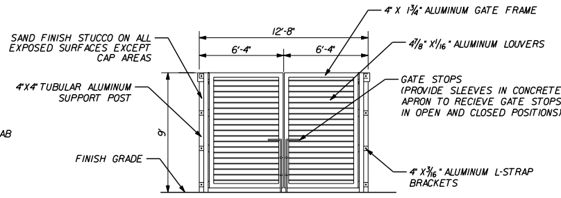
FRONT GATE ELEVATION
