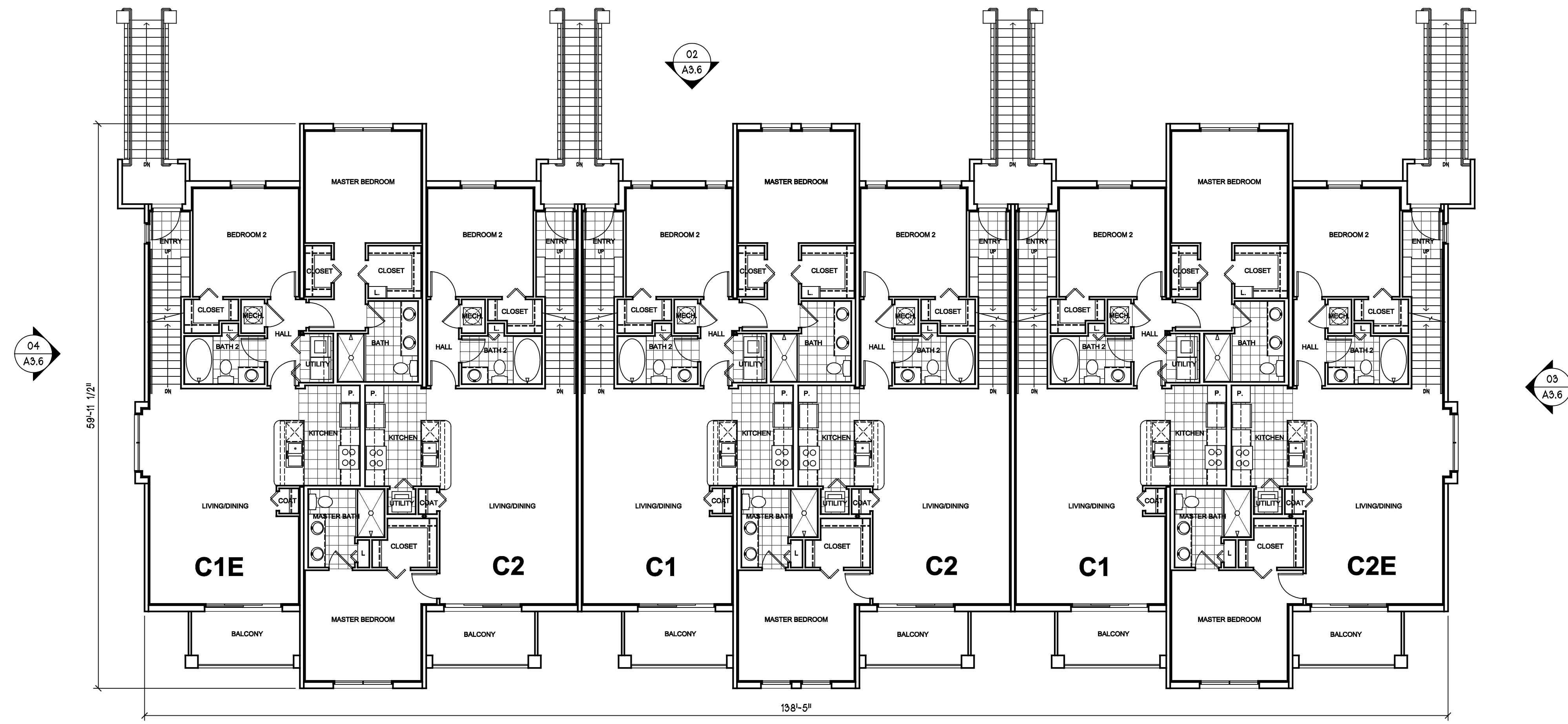
02 SECOND FLOOR - BUILDING TYPE II (BUILDINGS NO. 1 & 8) 1/8" = 1'- 0"
