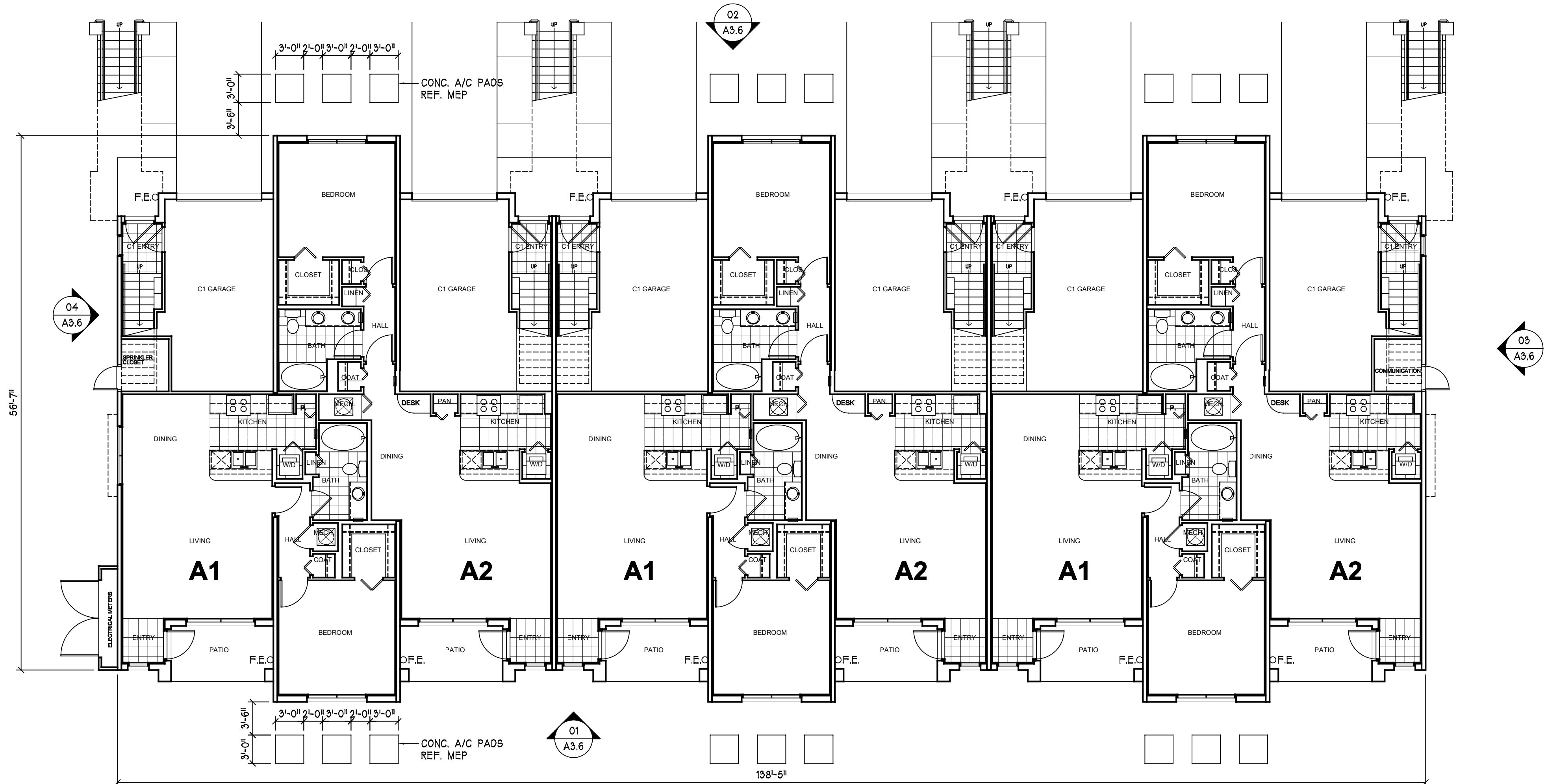
01 FIRST FLOOR - BUILDING TYPE II (BUILDINGS NO. 1 & 8) 1/8" = 1'- 0"
