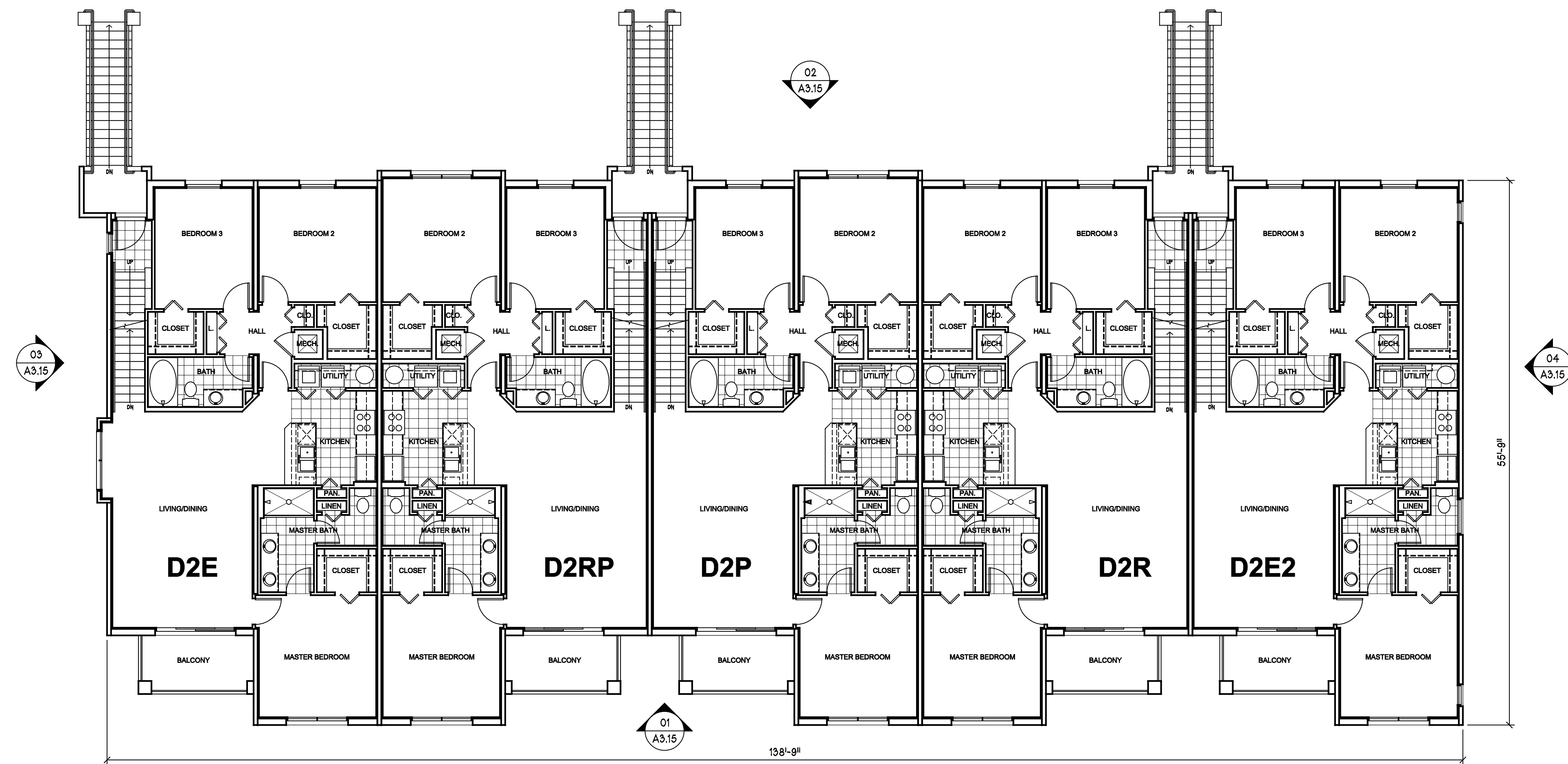
02 SECOND FLOOR - BUILDING TYPE V (BUILDING NO. 6) 1/8" = 1'-0"
