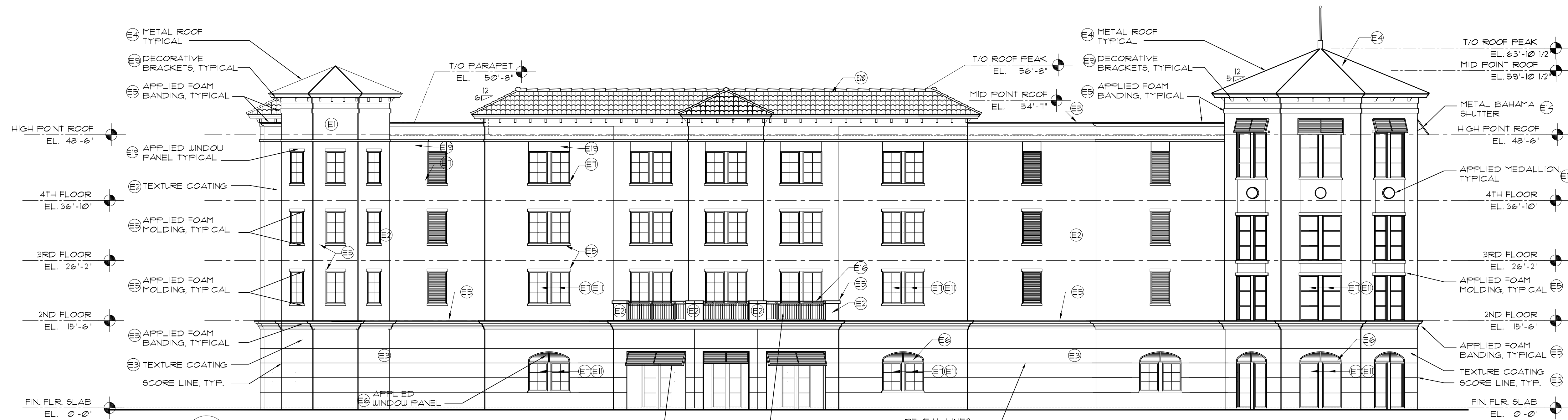
1 SOUTH (WILES ROAD) ELEVATION 3/32"=1'-0"
