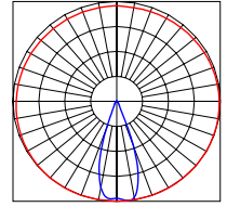
Polar Curve
