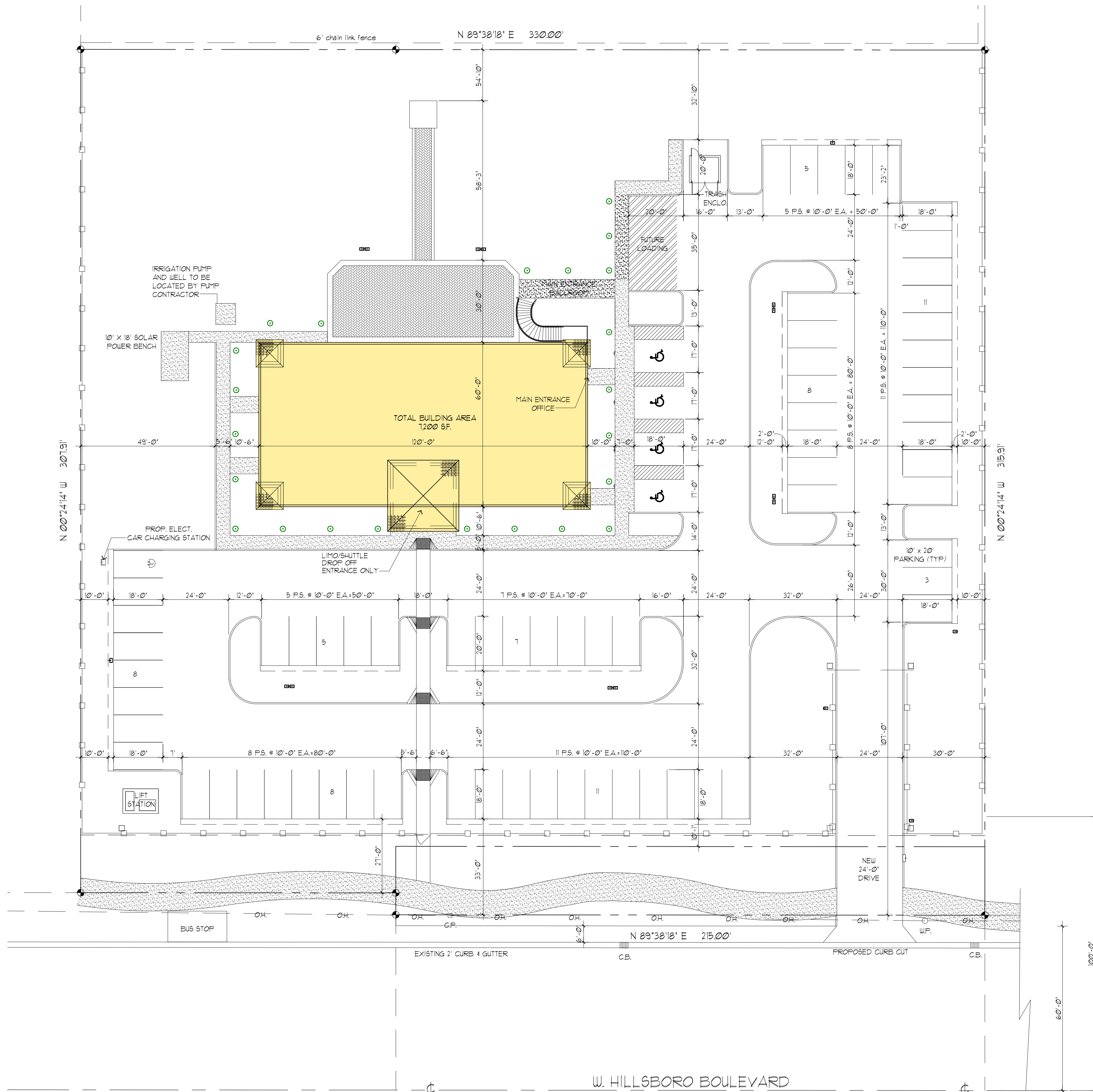
Site Plan 1" = 20'
