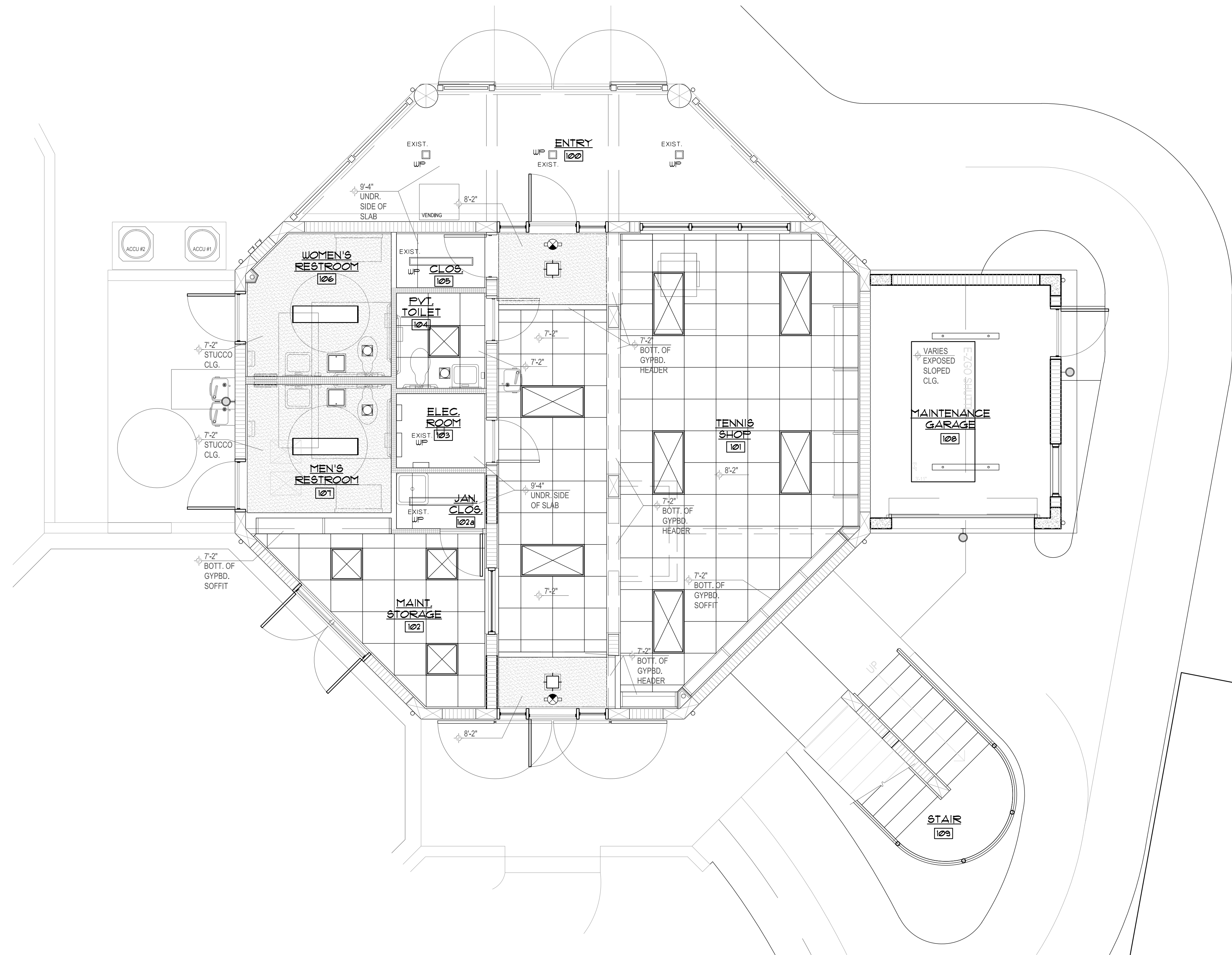
1 GROUND FLOOR REFLECTED CEILING PLAN 1/4" = 1'-0"
