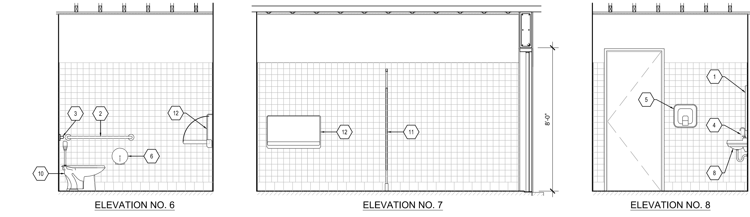
2 RESTROOM 101 ELEVATION SCALE : 3/8" = 1'-0"
