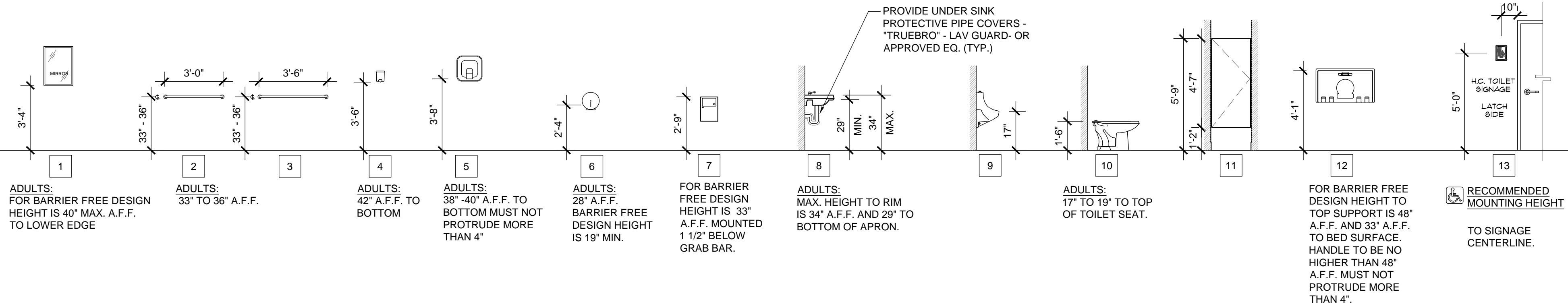
4 TOILET ACCESSORY MOUNTING HEIGHTS SCALE : 1/4" = 1'-0"
