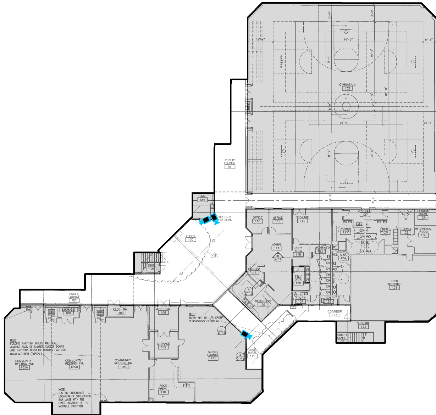
COMMUNITY CENTER - 1 st FLOOR PLAN
