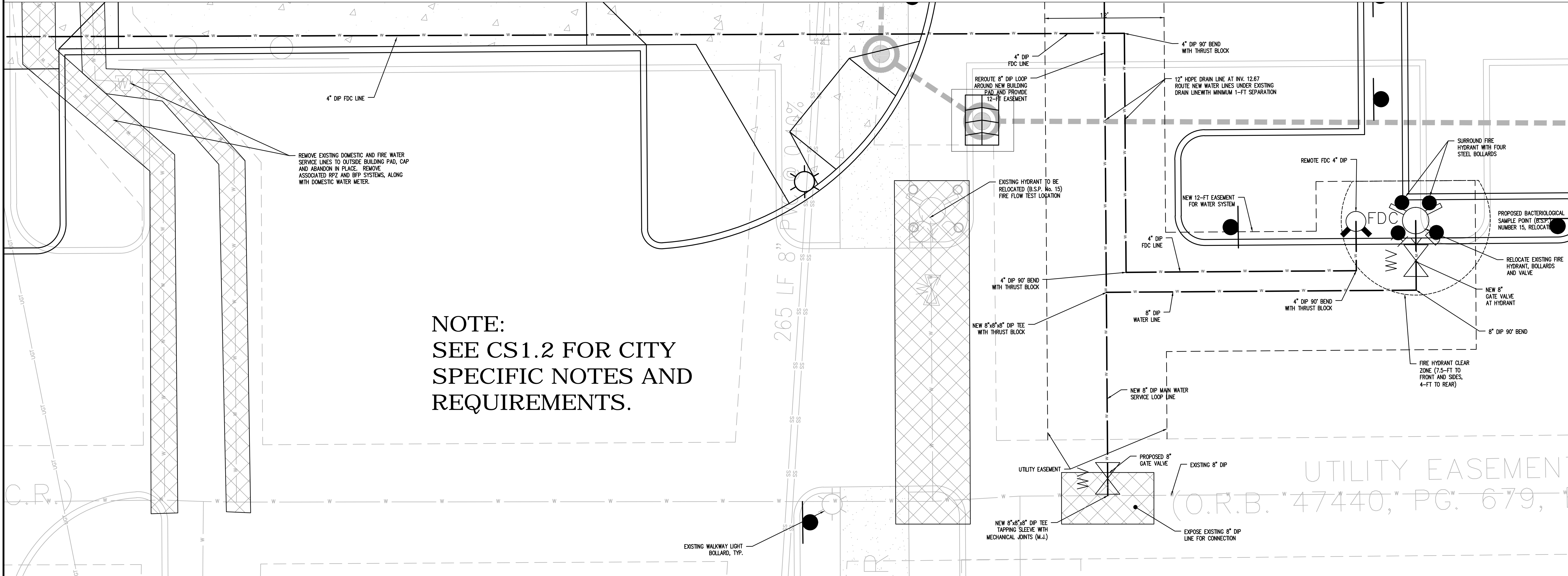
CONNECTIONS AT SOUTHEAST CORNER OF BUILDING
